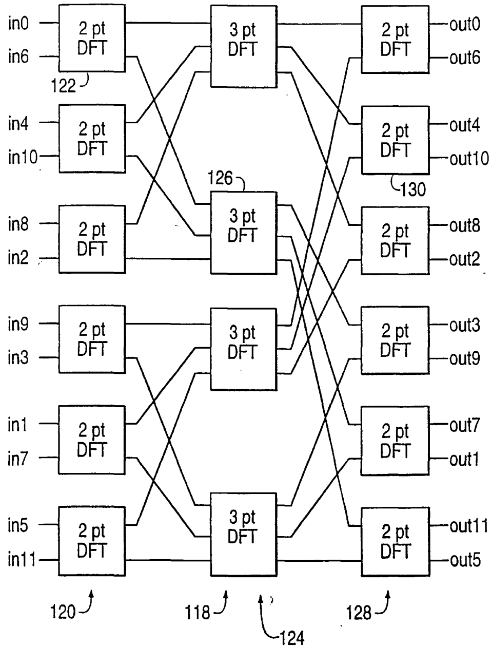
FIG. 8 (PRIOR ART)
