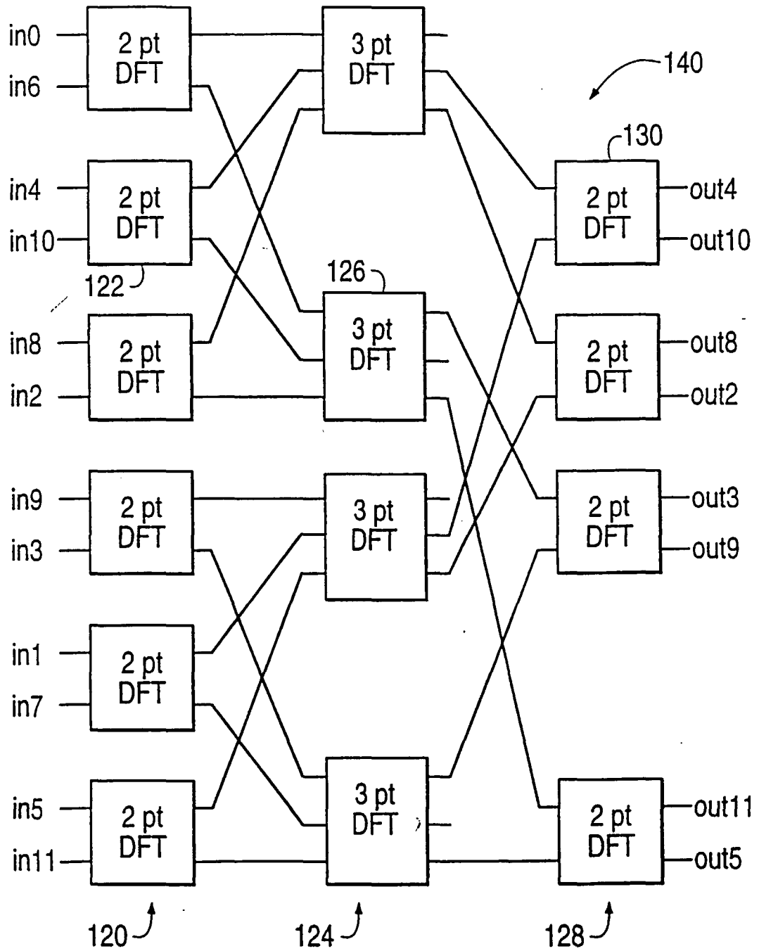
FIG. 9 (PRIOR ART)
