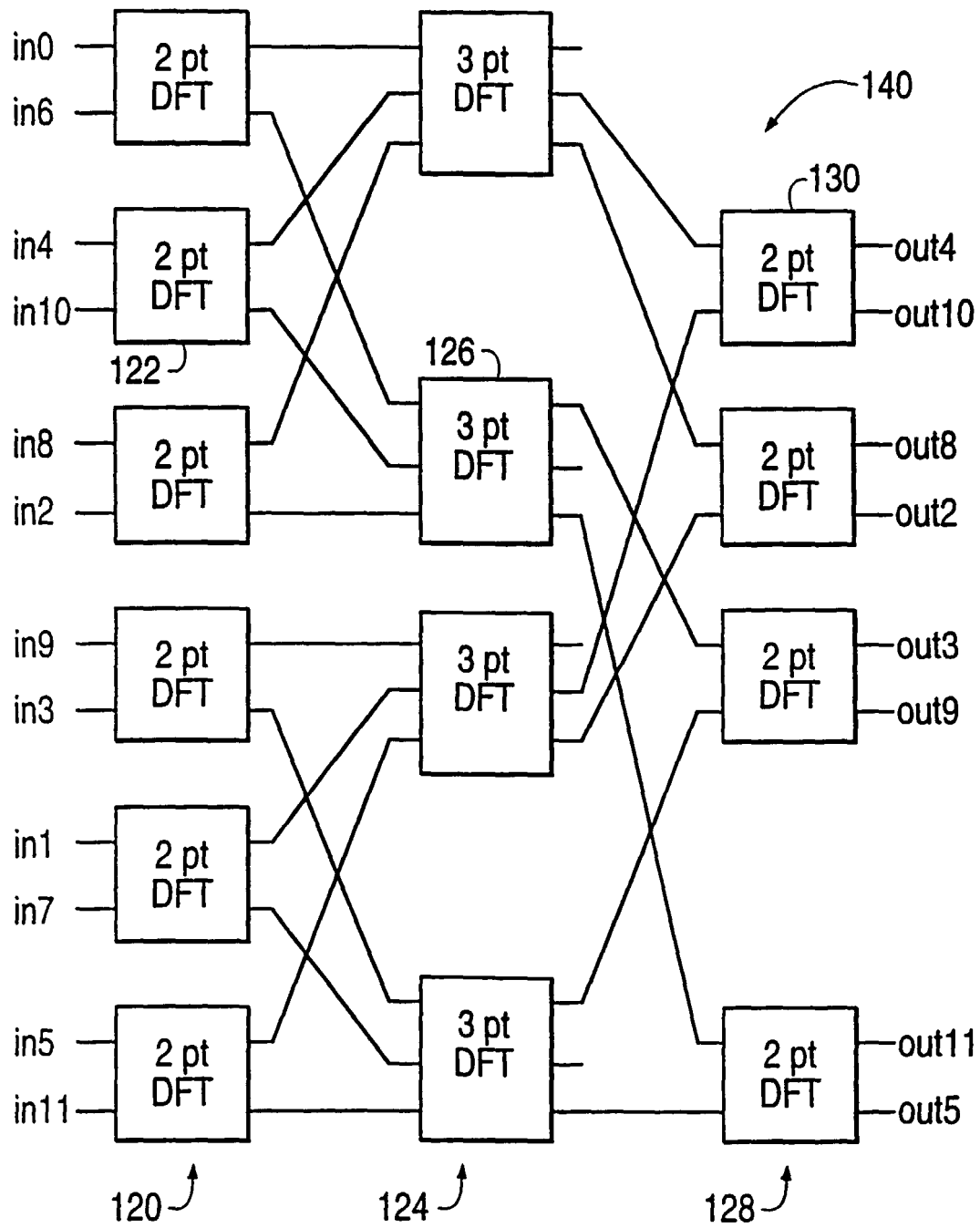
FIG. 9 (PRIOR ART)
