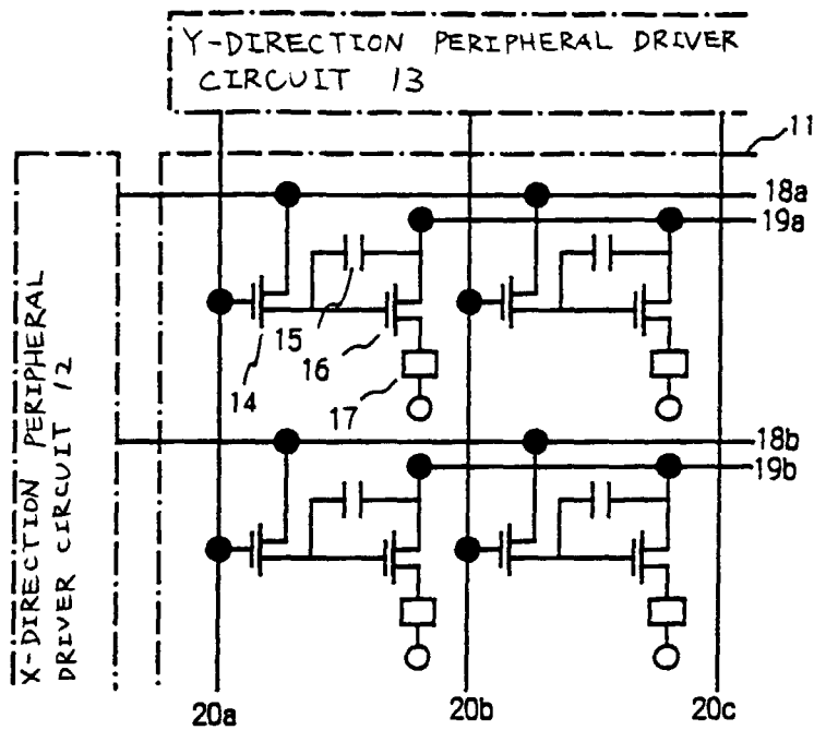
CIRCUIT DIAGRAM OF EL PANEL
