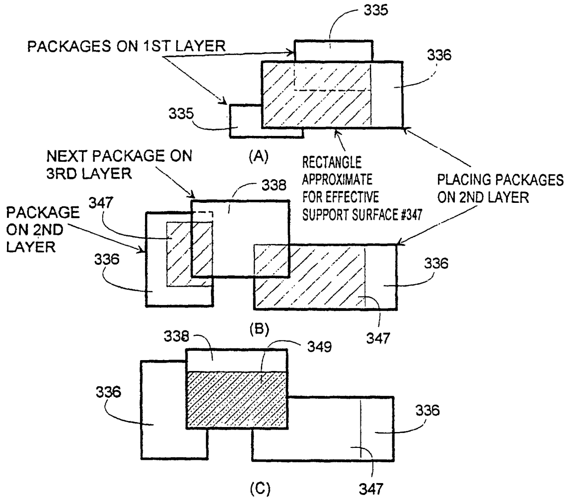
RECTANGLE APPROXIMATE FOR EFFECTIVE SUPPORT SURFACE
