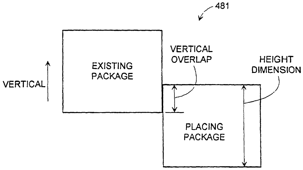
FRONT VIEW FIG. 48A
