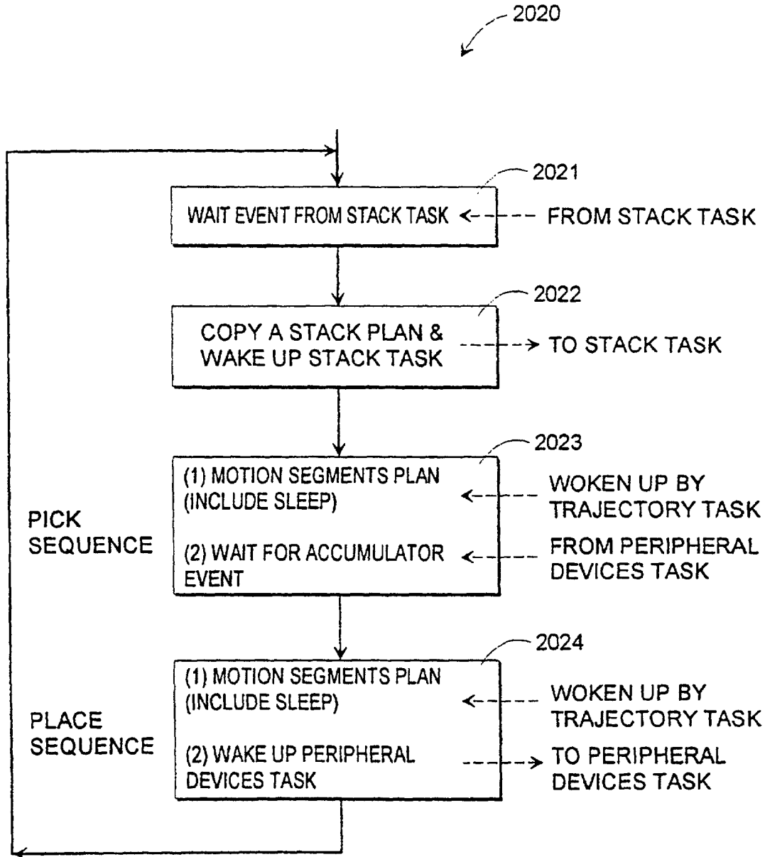
PLAN TASK EXECUTION FLOW CHART
