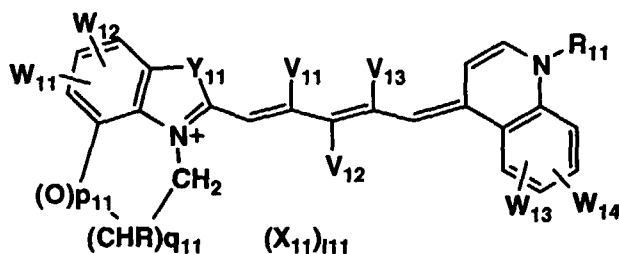
Formula (2)
