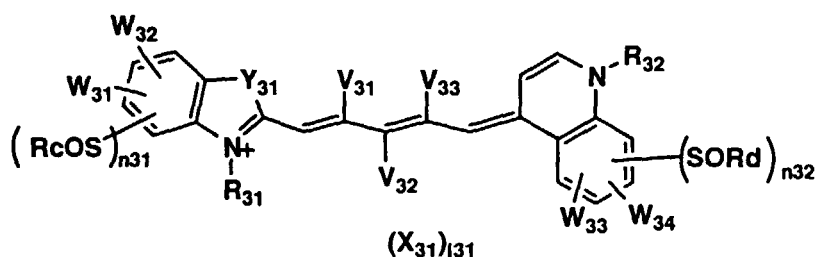
Formula (4)
