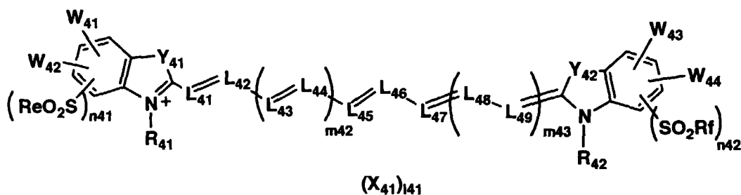
Formula (5)
