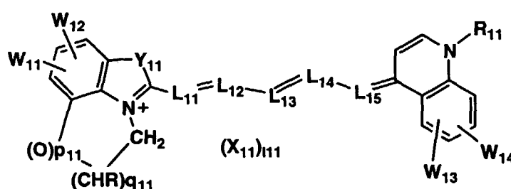
Formula (2-1)
