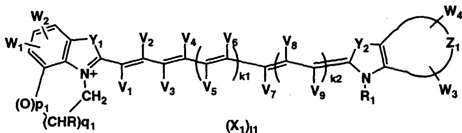
Formula (1)
