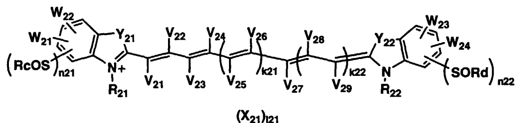
Formula (4)
