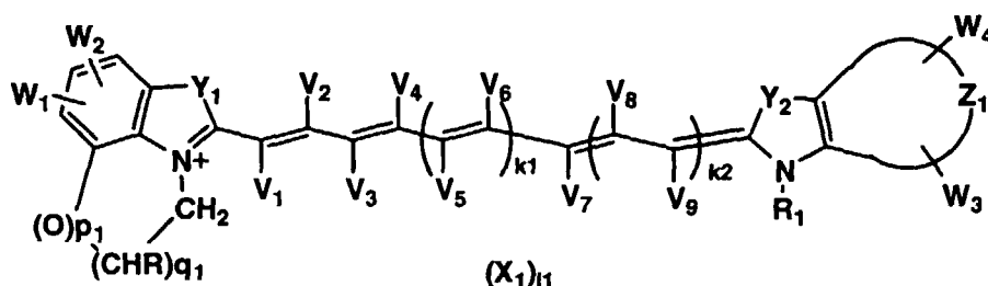
Formula (2)
