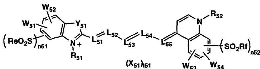
Formula (6)
