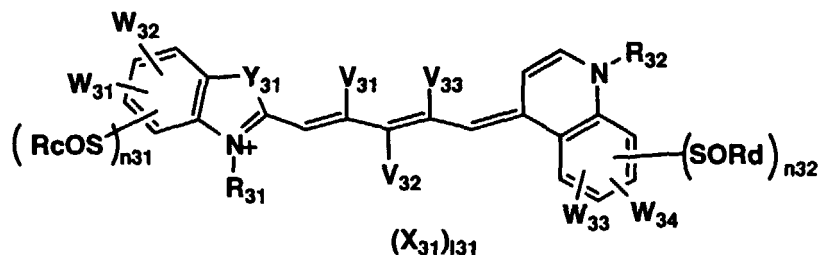
Formula (4)
