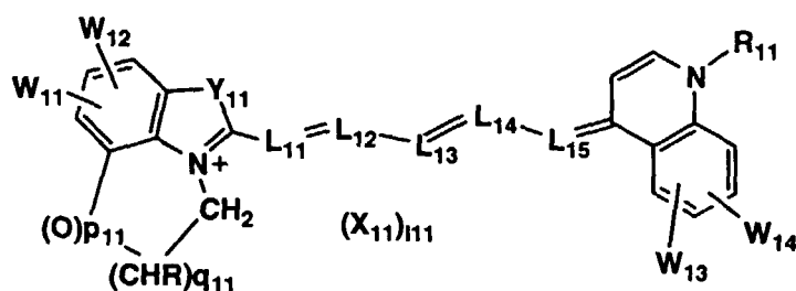
Formula (2-1)
