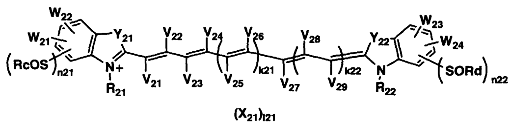
Formula (3)
