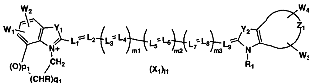
Formula (2-1)
