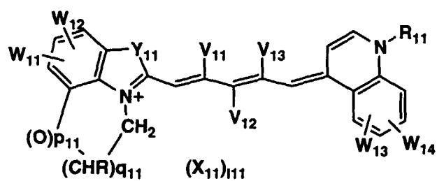
Formula (3)
