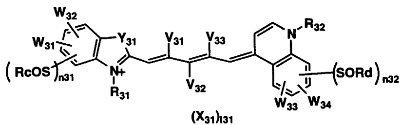
Formula (4)
