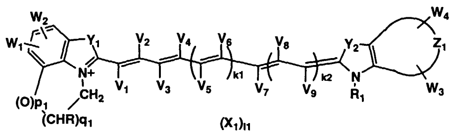
Formula (2)
