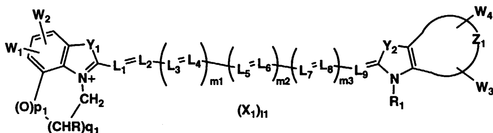
Formula (2-1)
