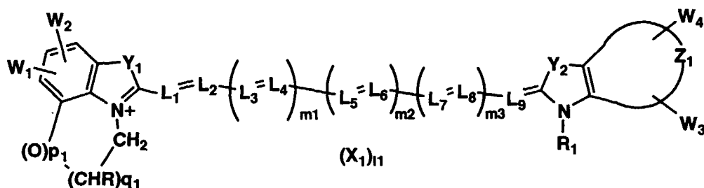
Formula (1-1)
