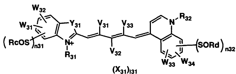
Formula (4)
