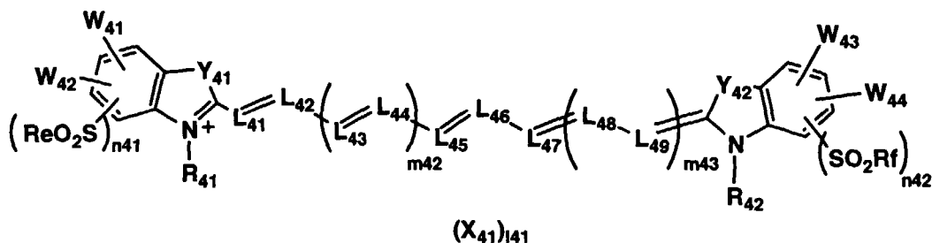
Formula (5)
