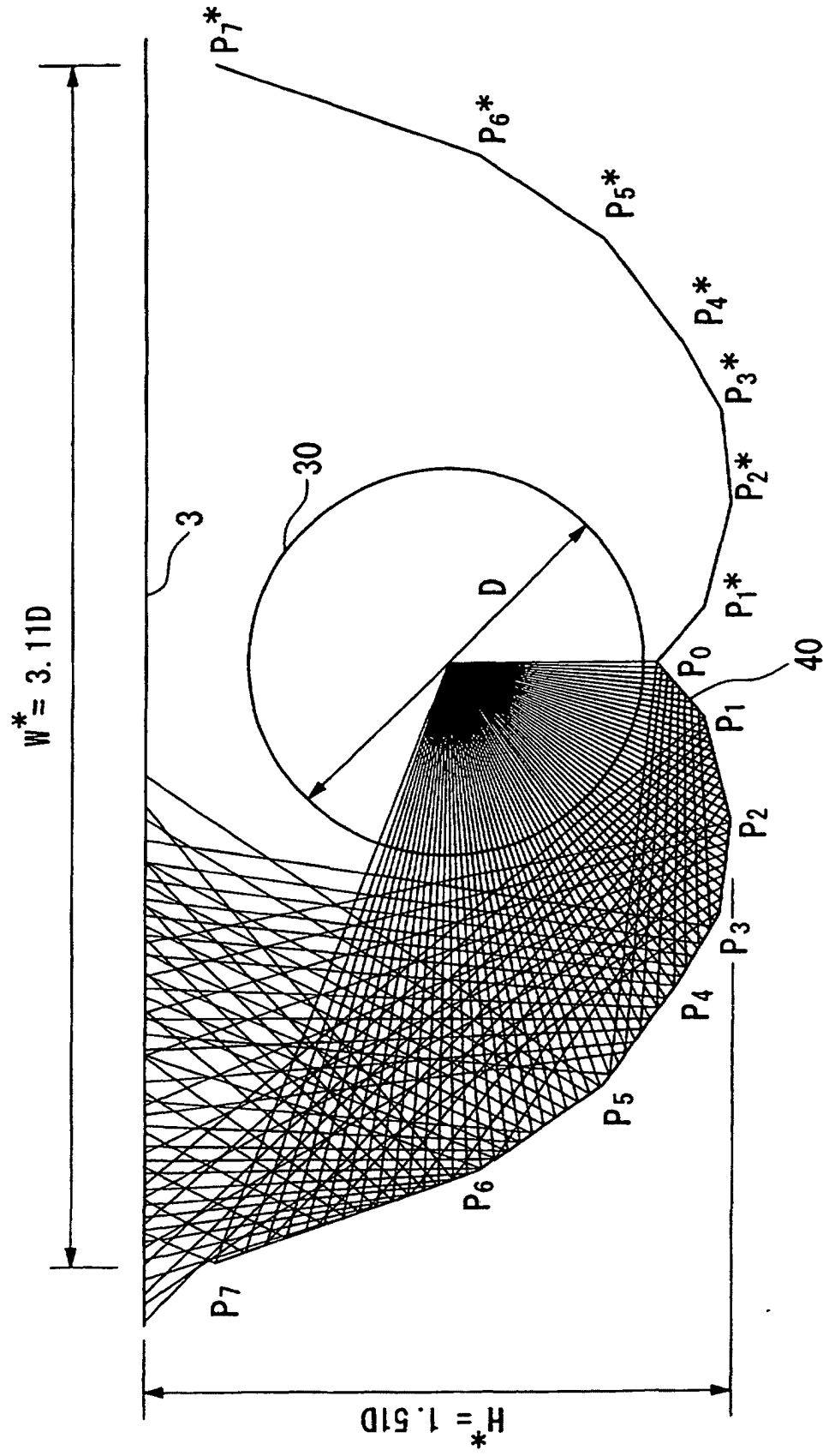
FIG. 6 Prior Art
