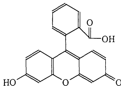
Fluorescein
