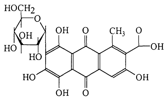
Carminic Acid
