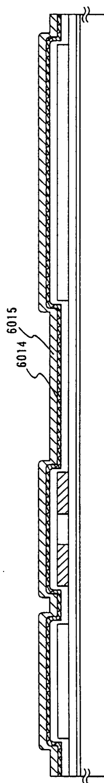
Fig. 8B (Formation of n-region)
