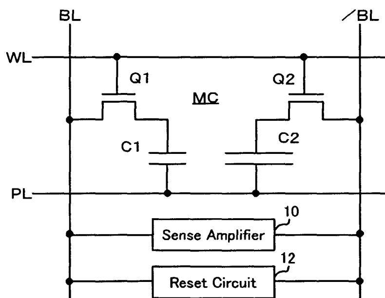
FIG. 1 2T2C Cell according to the Present Invention
