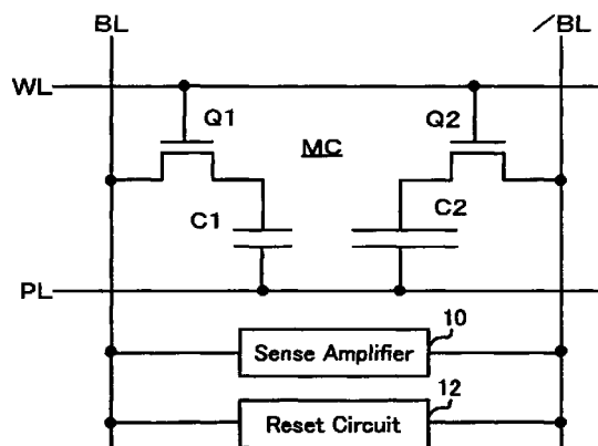
FIG. 1 2T2C Cell according to the Present Invention
