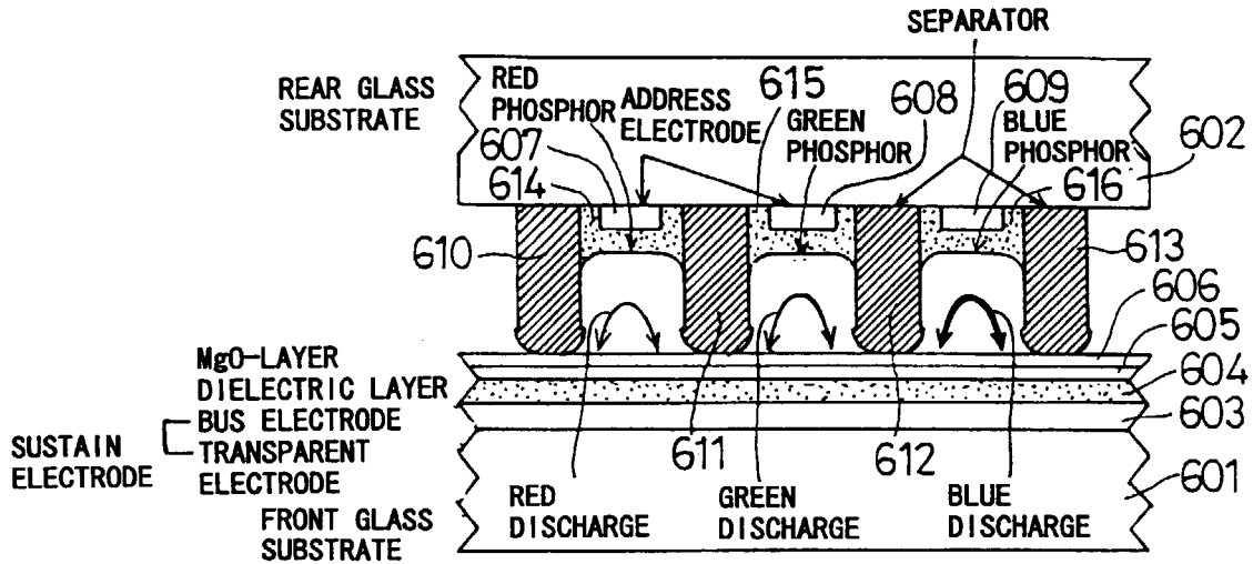
(A) CROSS SECTION OF PDP
