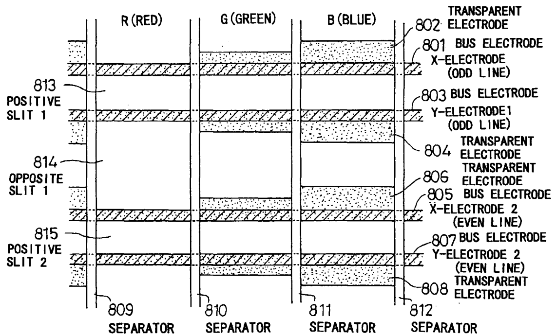
(A) PLAN VIEW OF SUSTAIN ELECTRODE
