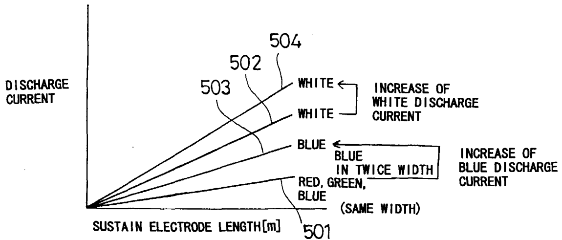
(A) RELATIONSHIP BETWEEN SUSTAIN ELECTRODE SIZE AND DISCHARGE CURRENT
