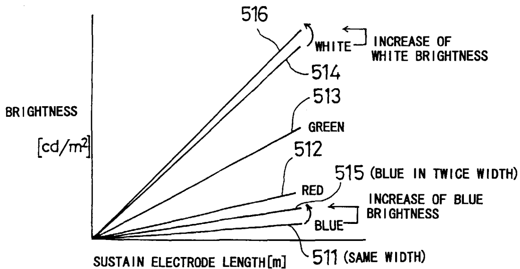
(B) RELATIONSHIP BETWEEN SUSTAIN ELECTRODE AREA AND BRIGHTNESS
