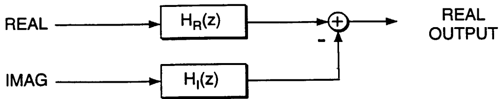
HALF-COMPLEX FILTER FIG. 6B
