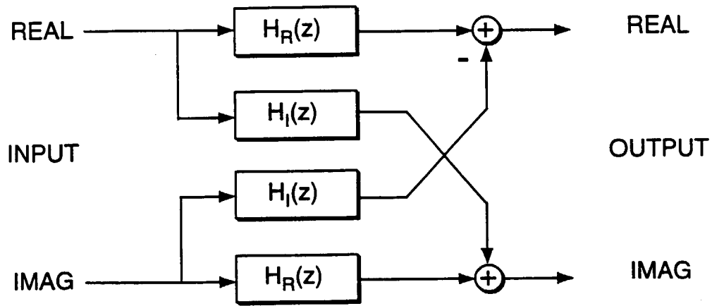
COMPLEX FILTER FIG. 6A
