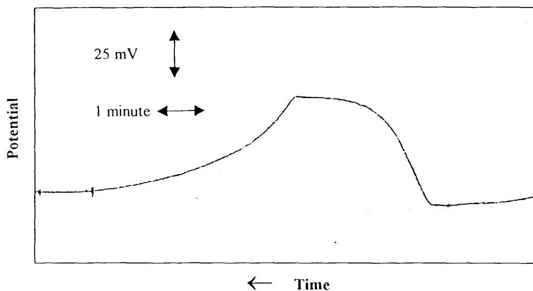
Figure 11 The time response to a step change in gaseous carbon dioxide in anhydrous air for a gas tight type carbon dioxide detection sensor B
