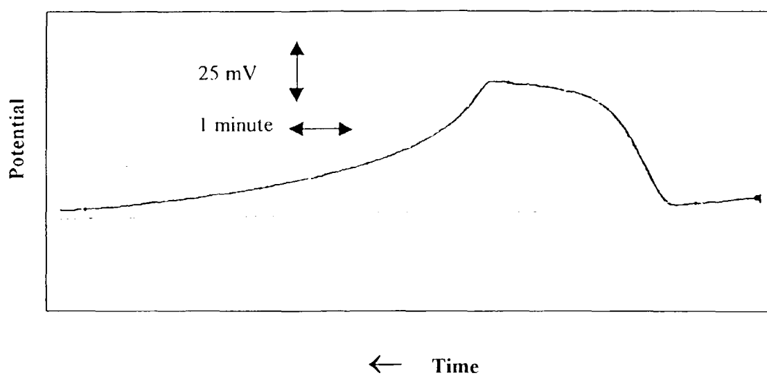
Figure 12 The time response to a step change in gaseous carbon dioxide in 60% humid air for a gas tight type carbon dioxide detection sensor B
