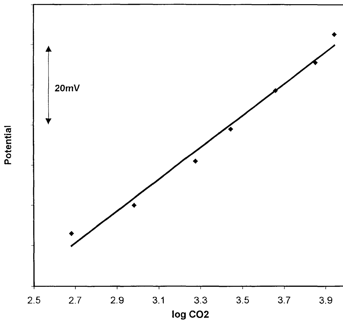
Figure 6 Cell Potential at 25 °C as a Function of the Log of the Carbon Dioxide Concentration in Anhydrous Air for Open Gas Type Carbon Dioxide Detection Sensor A
