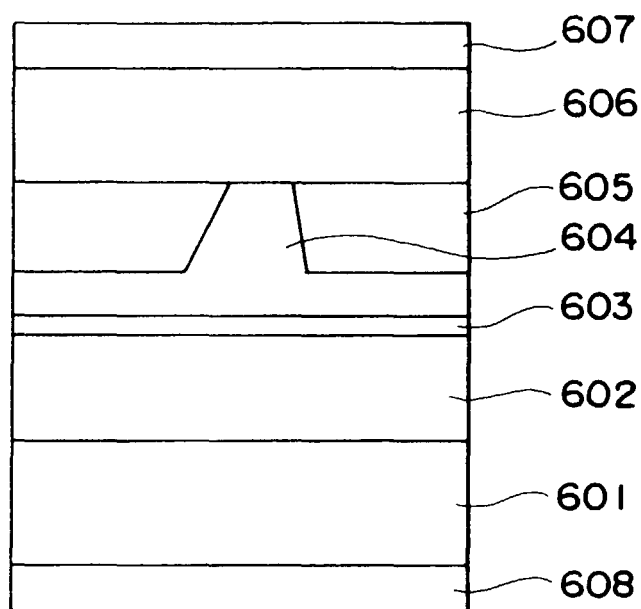
( a ) Ridge type
