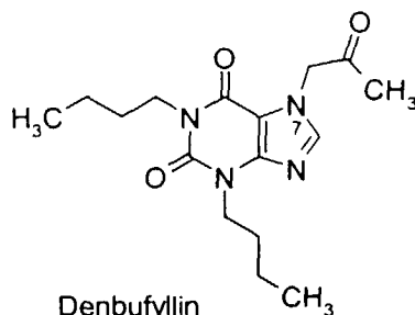
Denbufyllin
