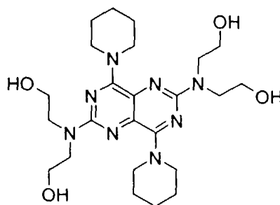
Dipyridamole
