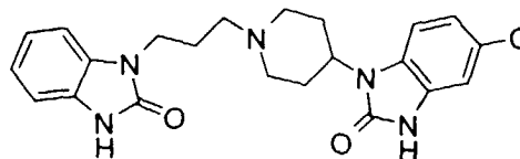
Domperidone
