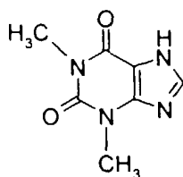
Theophylline
