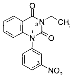
Nitraqazone
