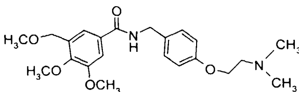
Tribenzomethamide
