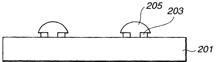
FIG.2C PRIOR ART
