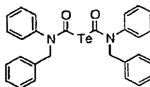
Tellurium Compound
