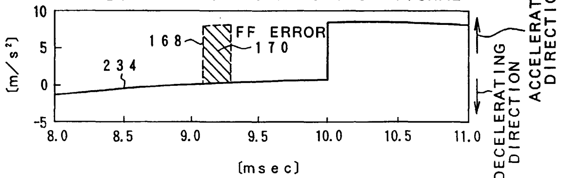
FIG. 31D DISTURBANCE COMPENSATION SIGNAL
