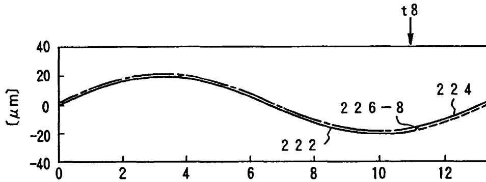
FIG. 33B POSITIONER SPEED
