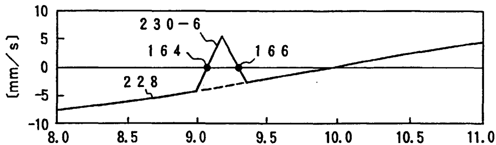
FIG. 31C TRACK JUMP SIGNAL
