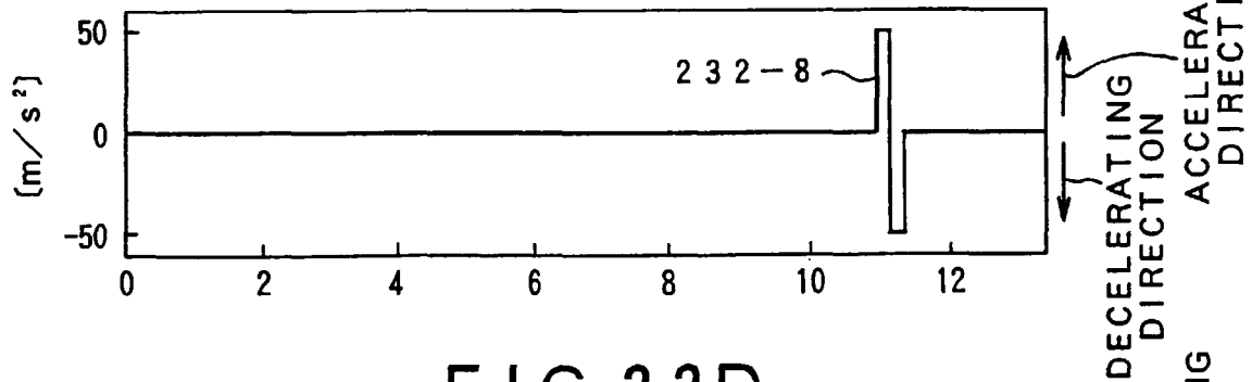
FIG. 33D DISTURBANCE COMPENSATION SIGNAL
