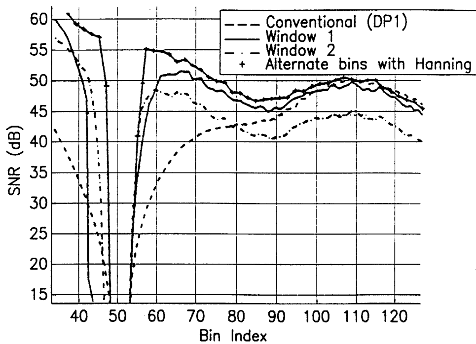
Medium Loop With NBI SNR Profile
