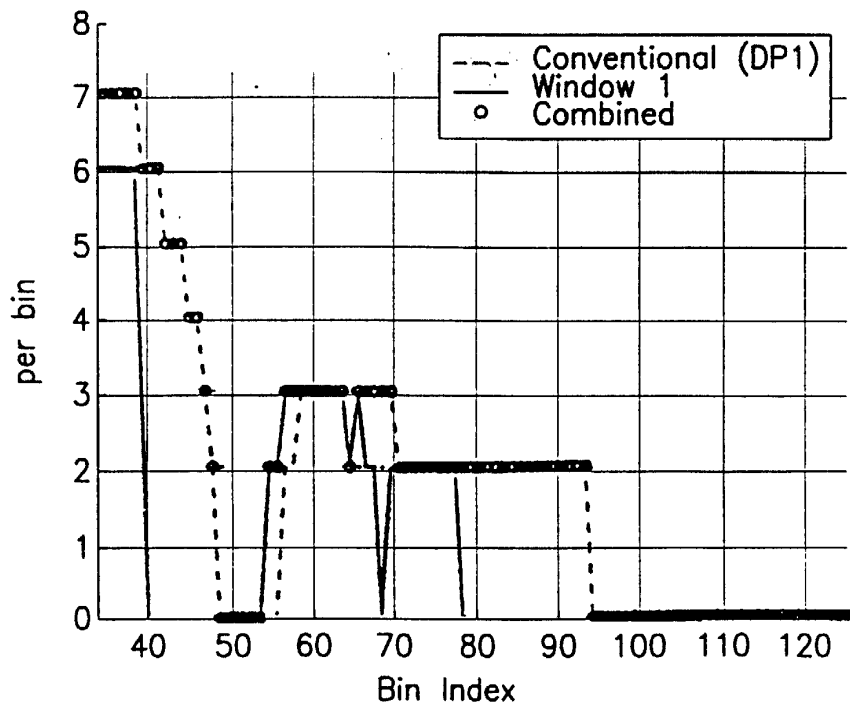
Long Loop With NBI Bit-Allocation Profile
