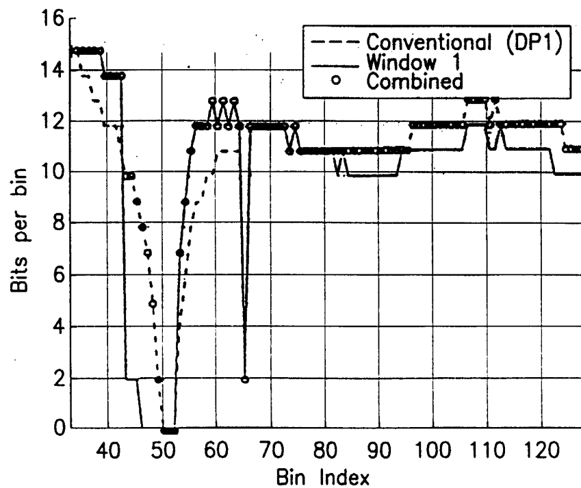
Medium Loop With NBI Bit-Allocation Profile
