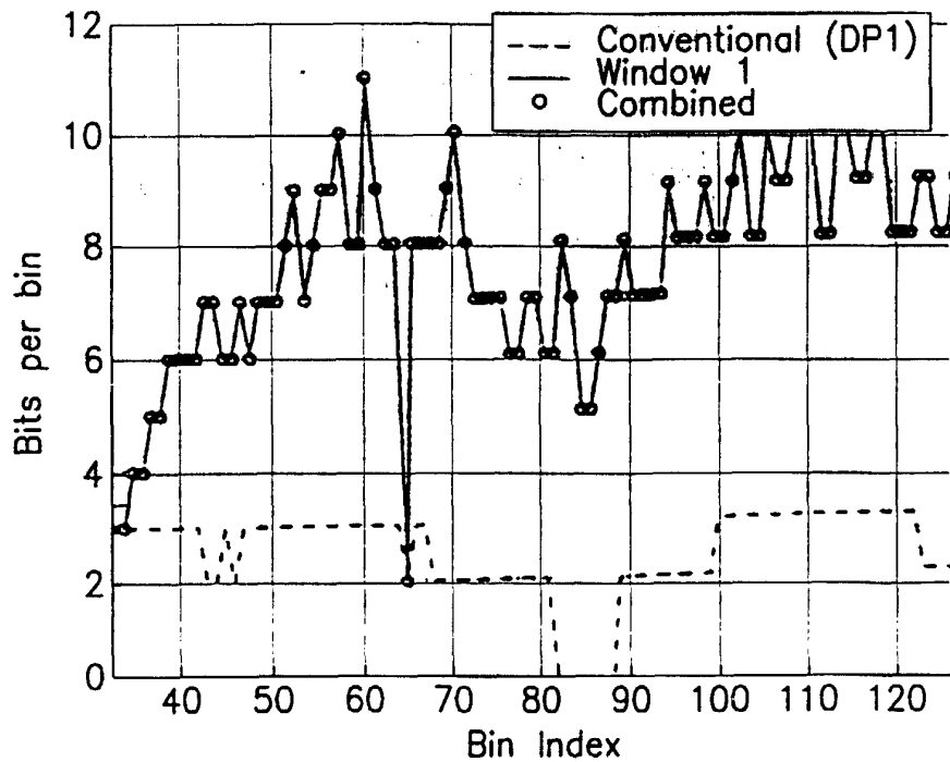
Medium Loop With Crosstalk Without TEQ Bit Allocation Profile
