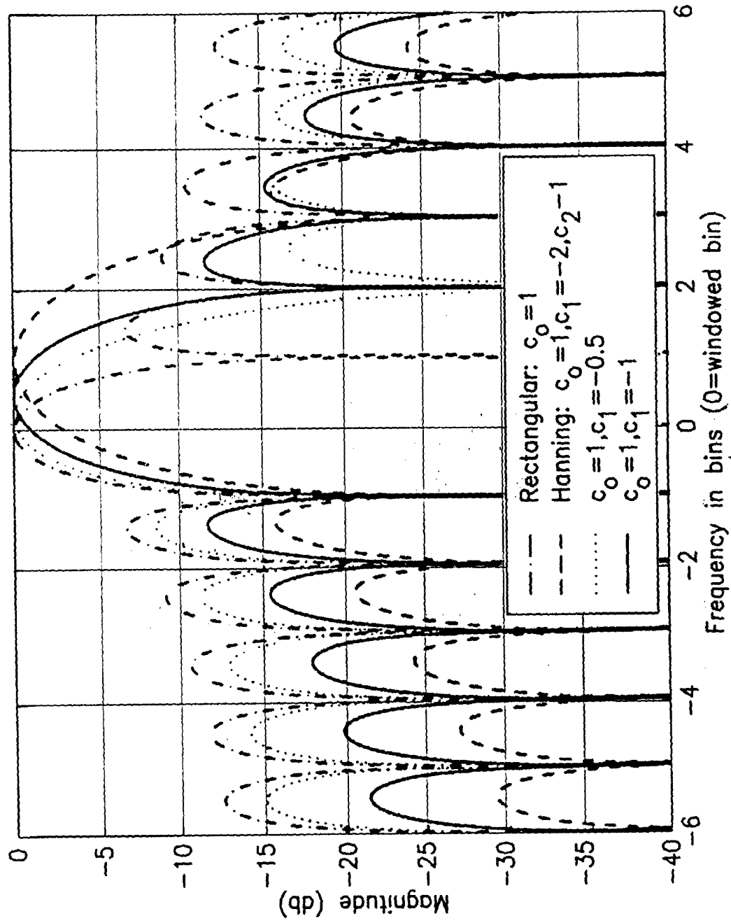
Different FDW Magnitude Responses
