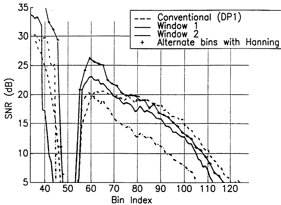
Long Loop With NBI Profile
