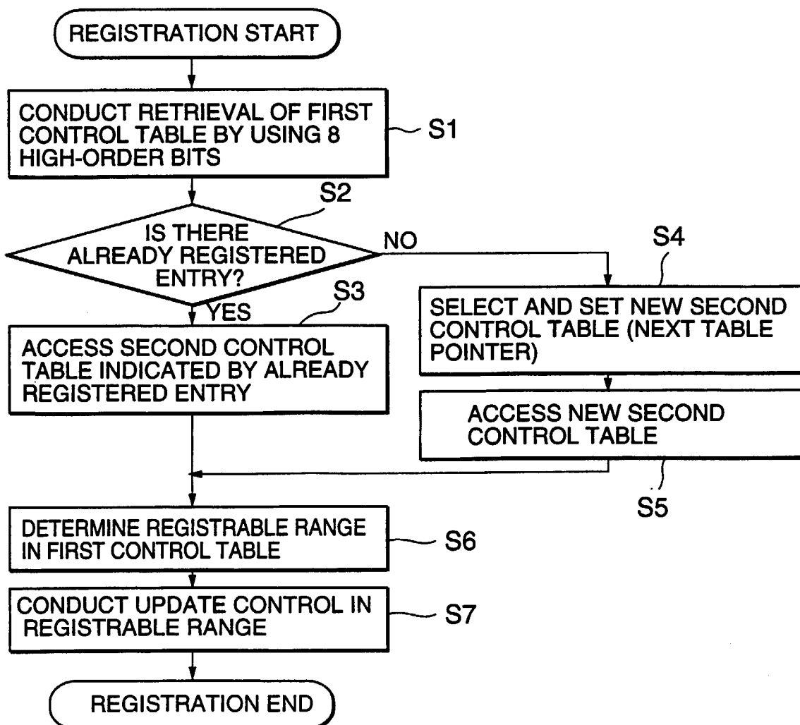
FIG.5 (PRIOR ART)
