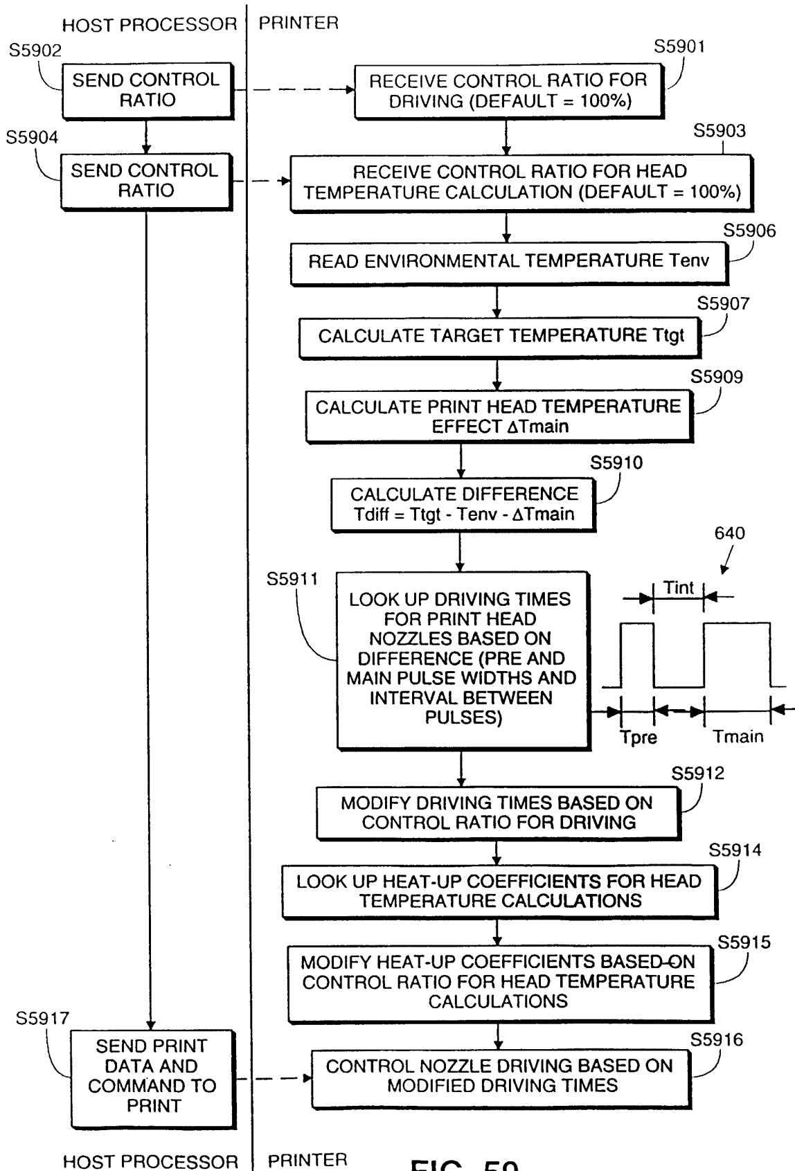
FIG. 59 PRIOR ART
