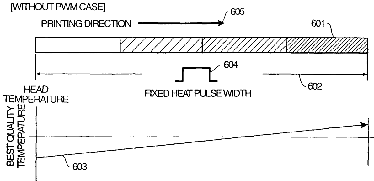
FIG. 57 (Prior Art)
