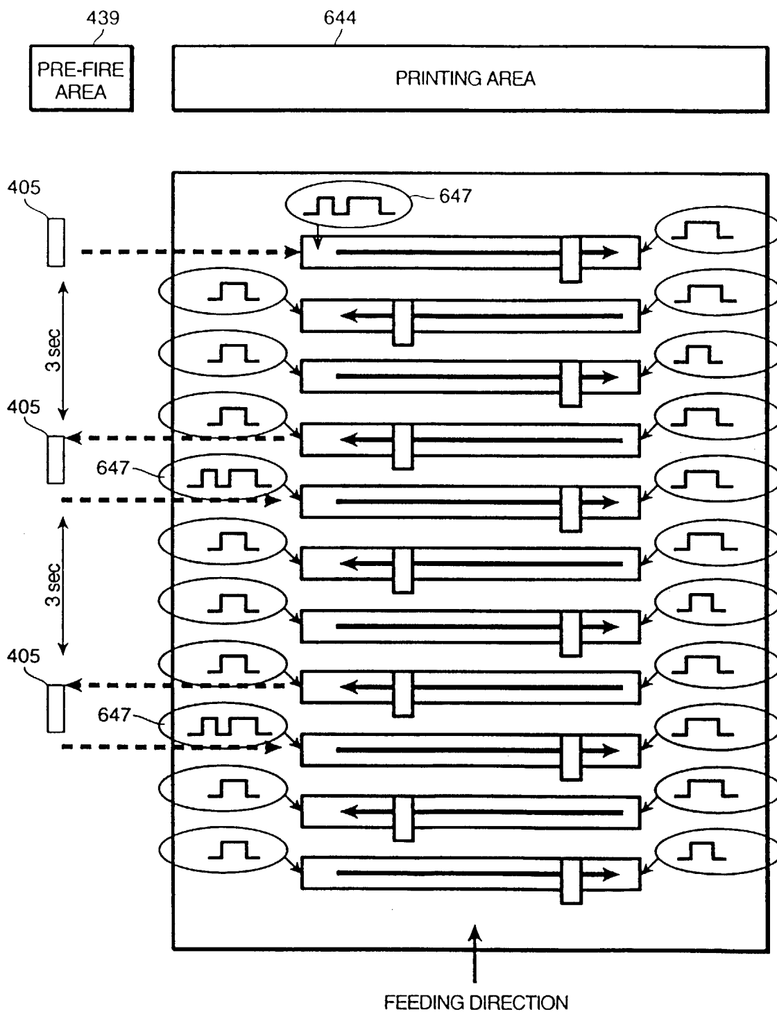
FIG. 62 (PRIOR ART)
