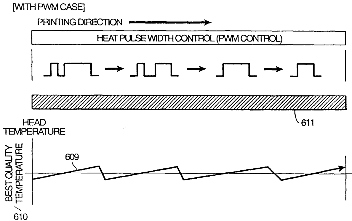
FIG. 58 (Prior Art)
