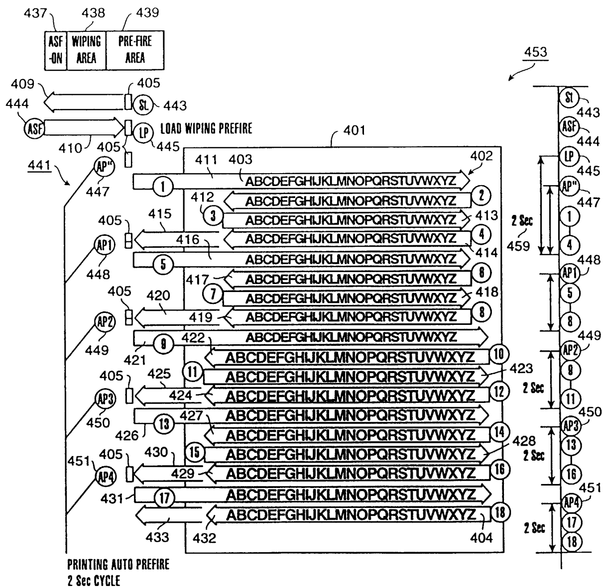
FIG. 47 (Prior Art)
