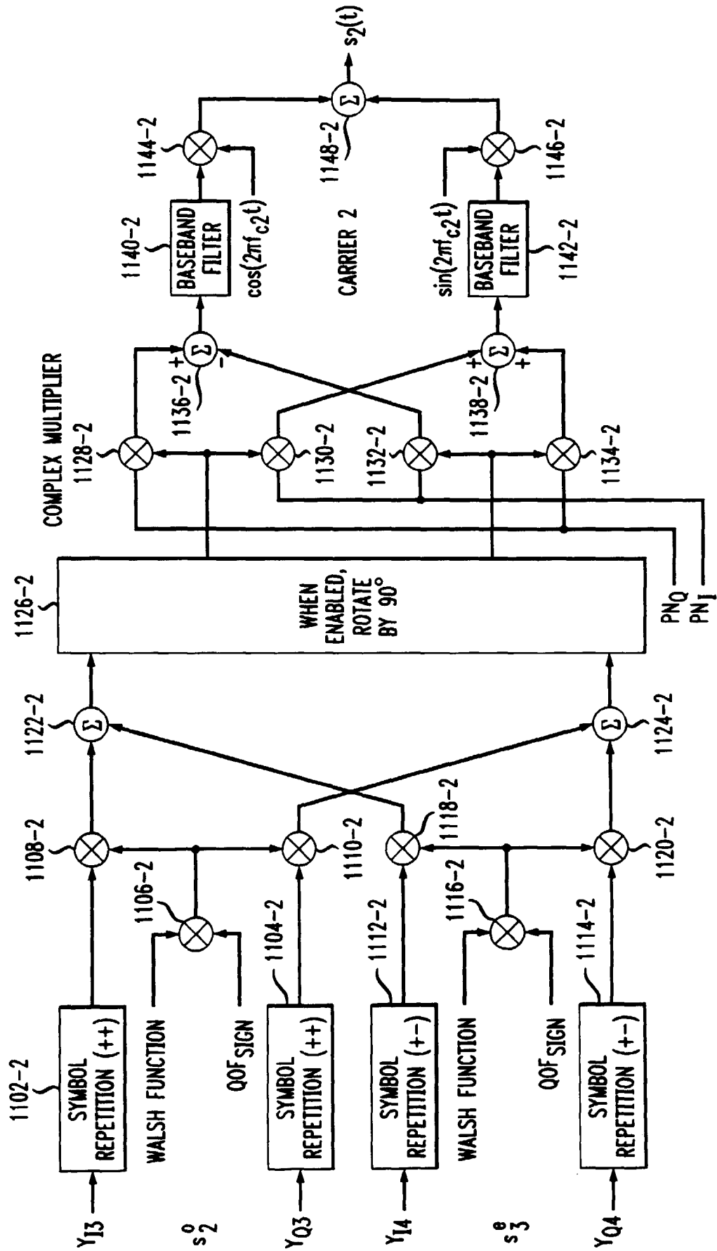
FIG. 11B P/O ANTENNA 1
