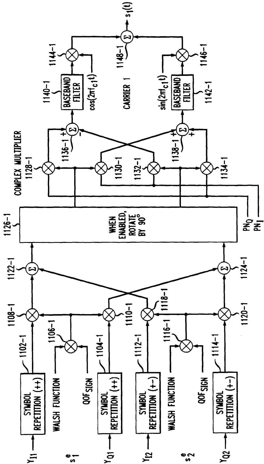
FIG. 11A P/O ANTENNA 1
