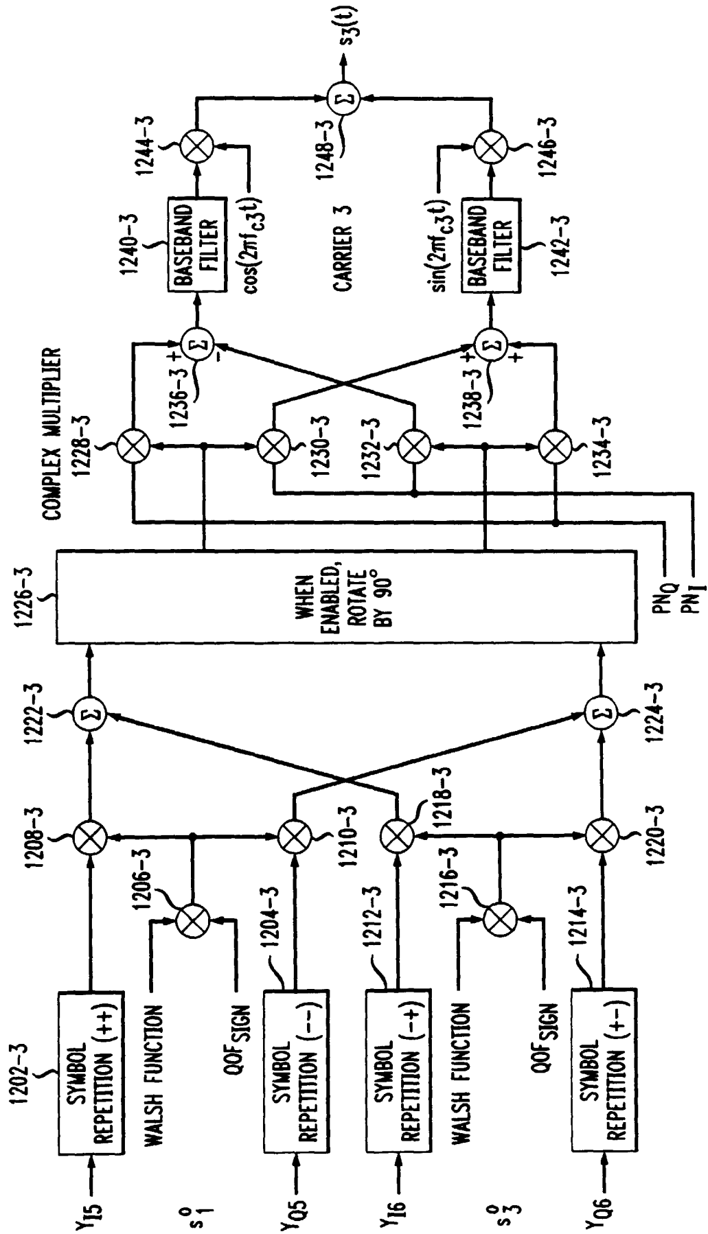
FIG. 12C P/O ANTENNA 2
