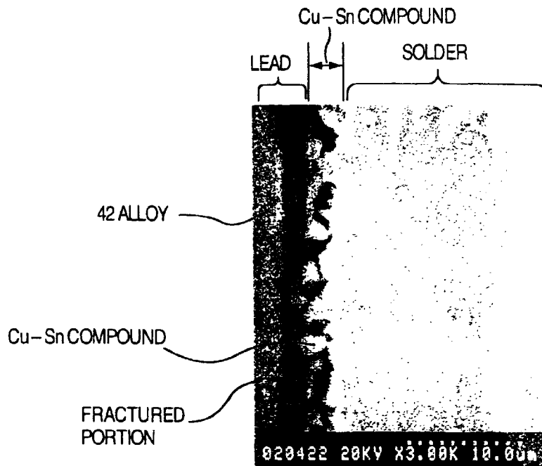
(a) SECTIONAL VIEW
