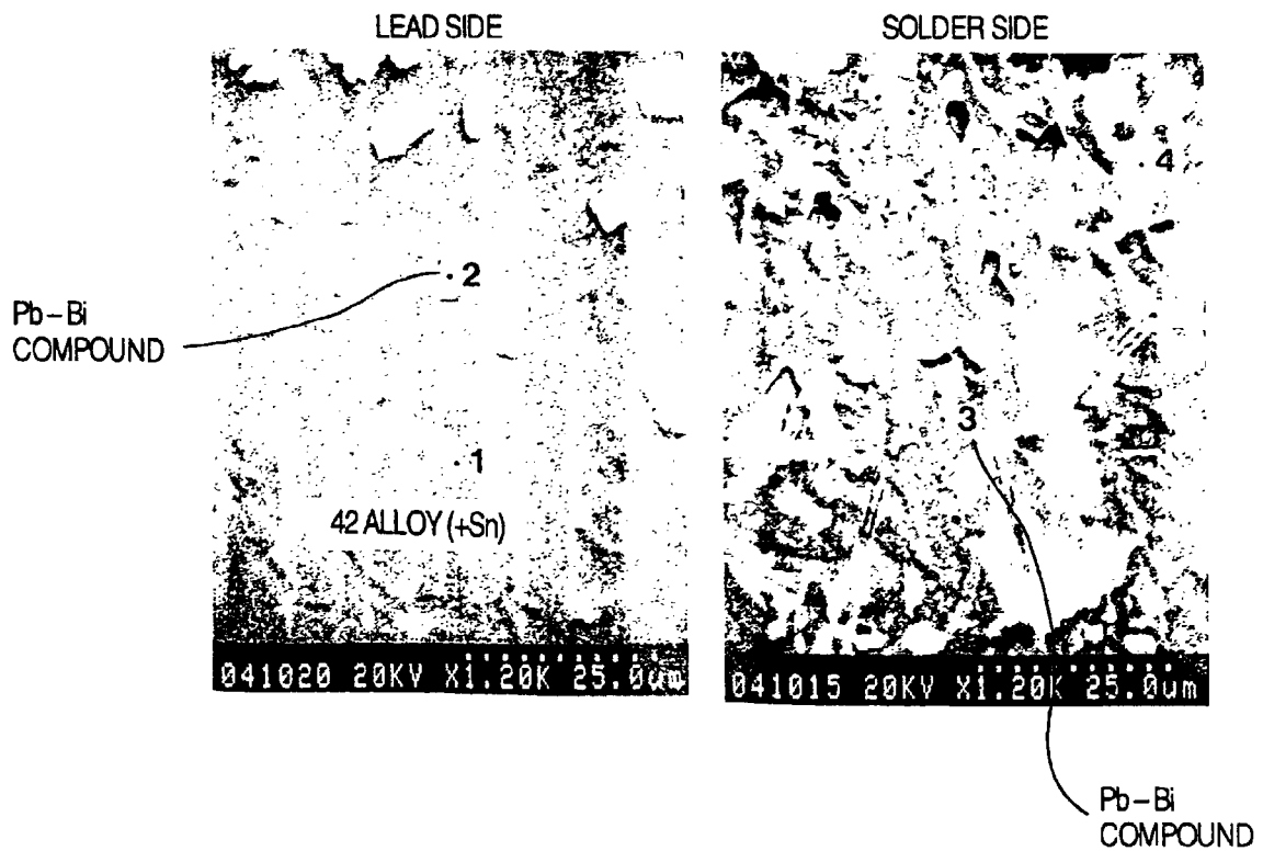
(b) FRACTURED PORTION
