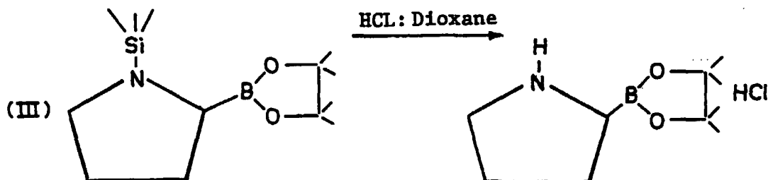
(IV) boroProline-pinacol-HCL
