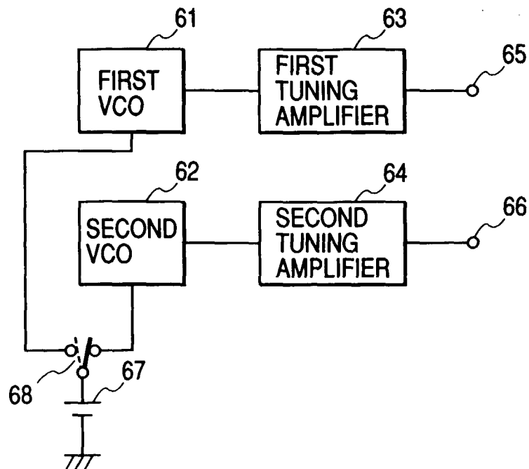
FIG. 6 PRIOR ART
