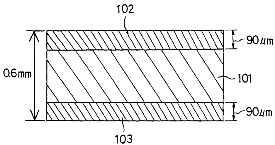
FIG. 15 PRIOR ART
