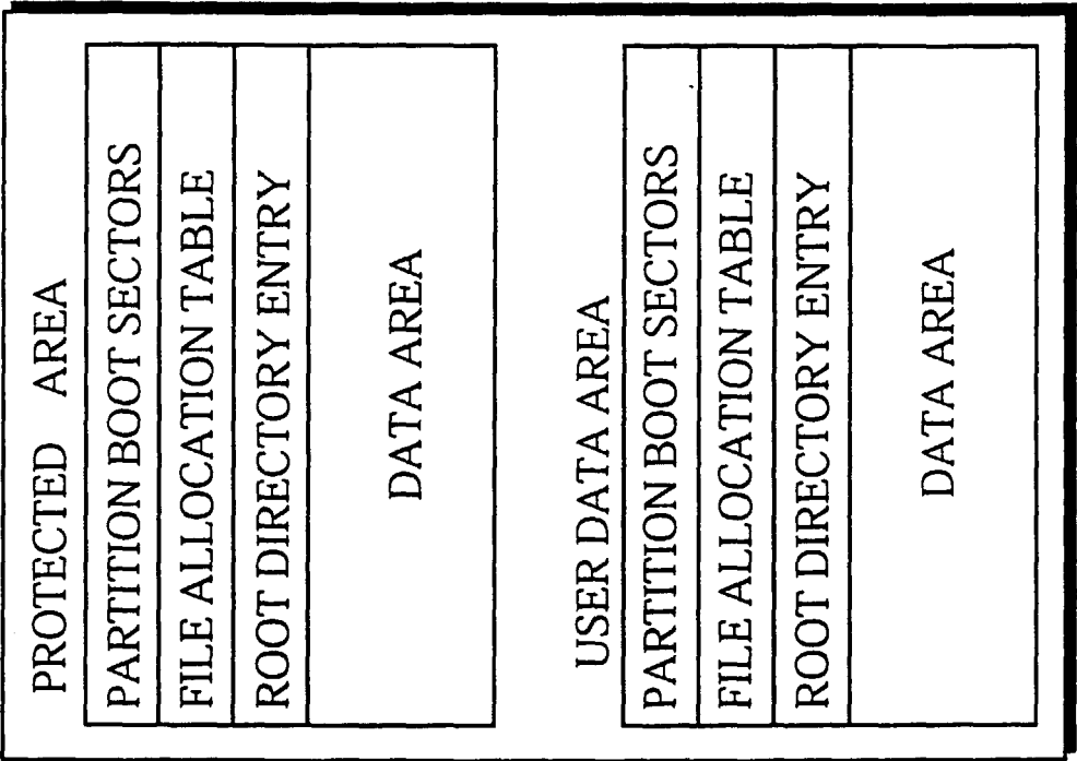
FIG. 4B FILE SYSTEM LAYER (ISO/IEC 9293)
