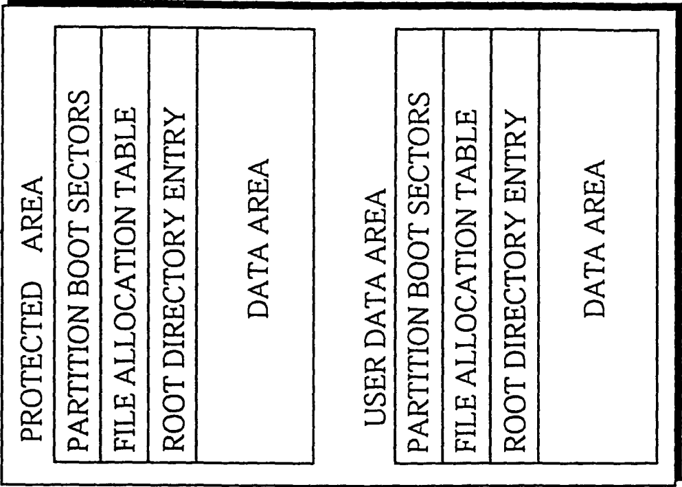
FIG. 4B FILE SYSTEM LAYER (ISO/IEC 9293)
