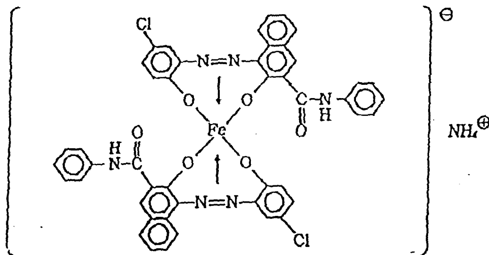
Monoazo dye Fe compound
