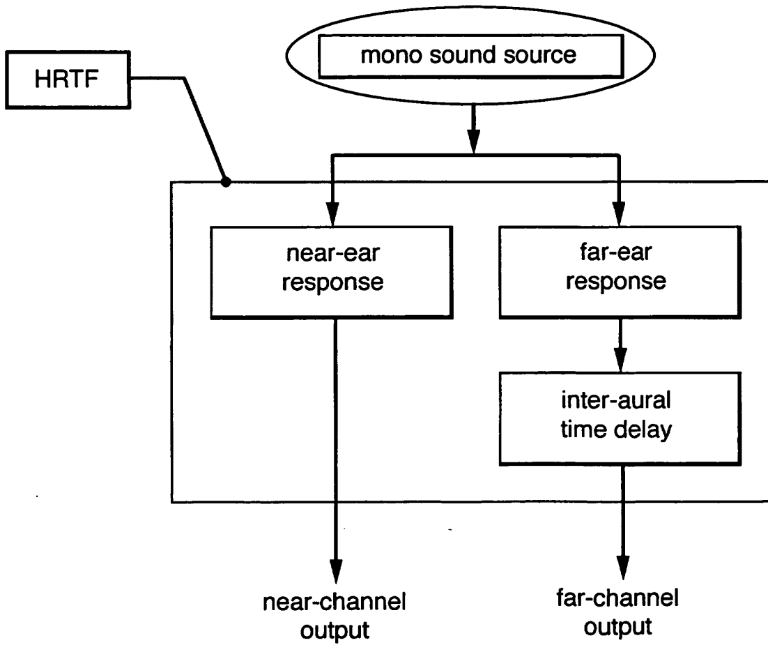
Fig.2. HRTF Processing diagram
