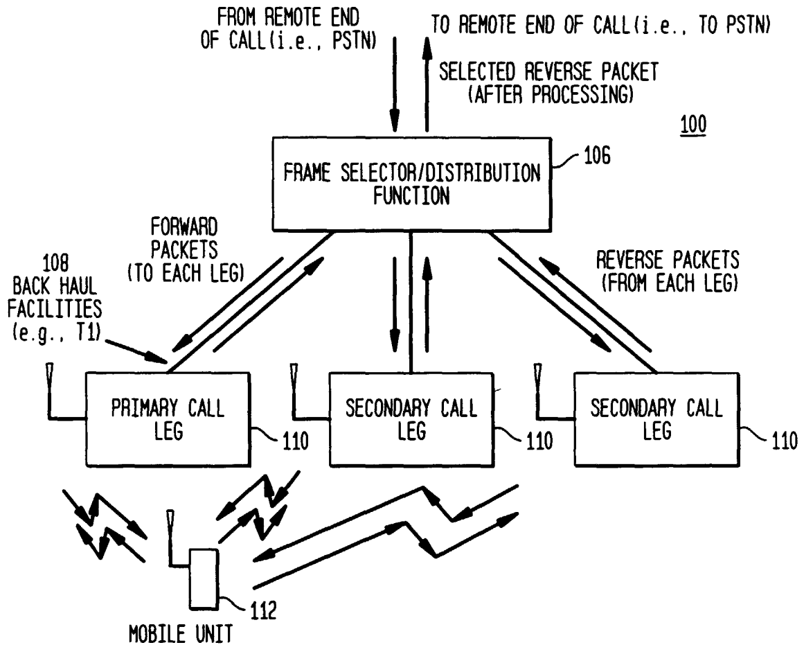
FIG. 2 (PRIOR ART)
