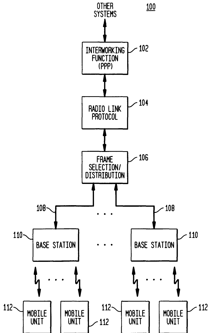
FIG. 1 (PRIOR ART)
