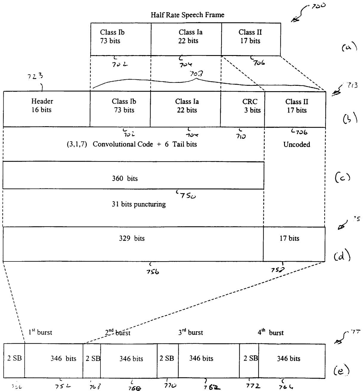
Figure 6. Channel coding for transmission of four speech frames in one RLC/MAC block - Uplink.
