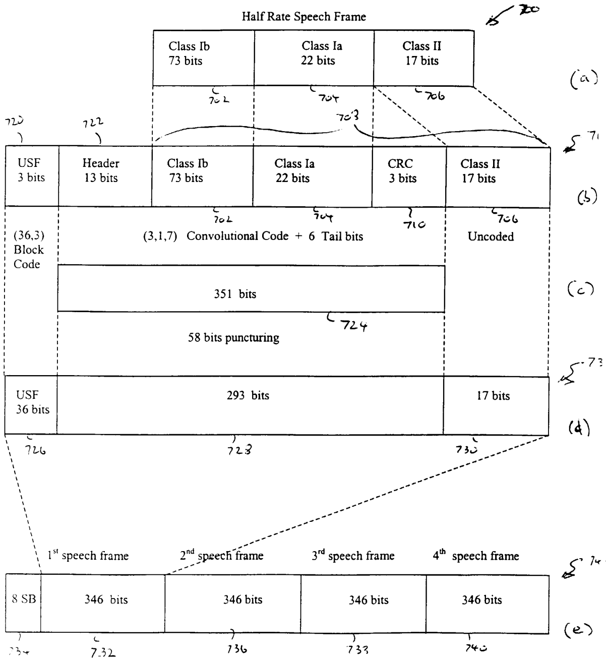
Figure 5. Channel coding for transmission of four speech frames in one RLC/MAC block – Downlink.
