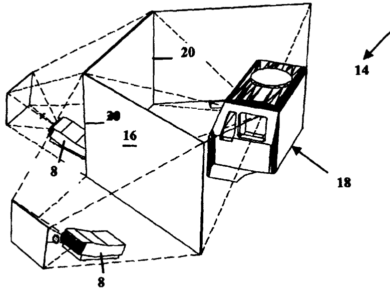
Figure 4: Rear-projected display for a truck simulator.
