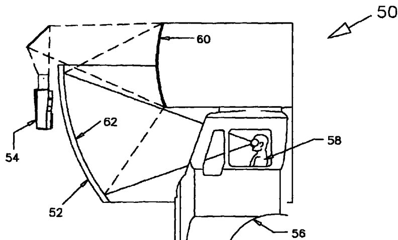
Figure 9: Front-projected PANORAMA side view
