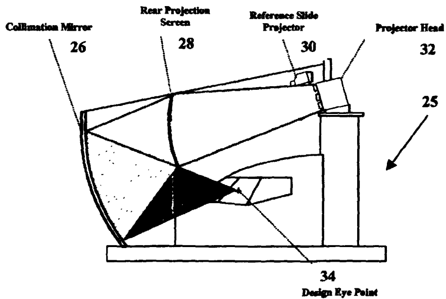
Figure 7: Tilted Mirror Collimation Flight Simulator Display
