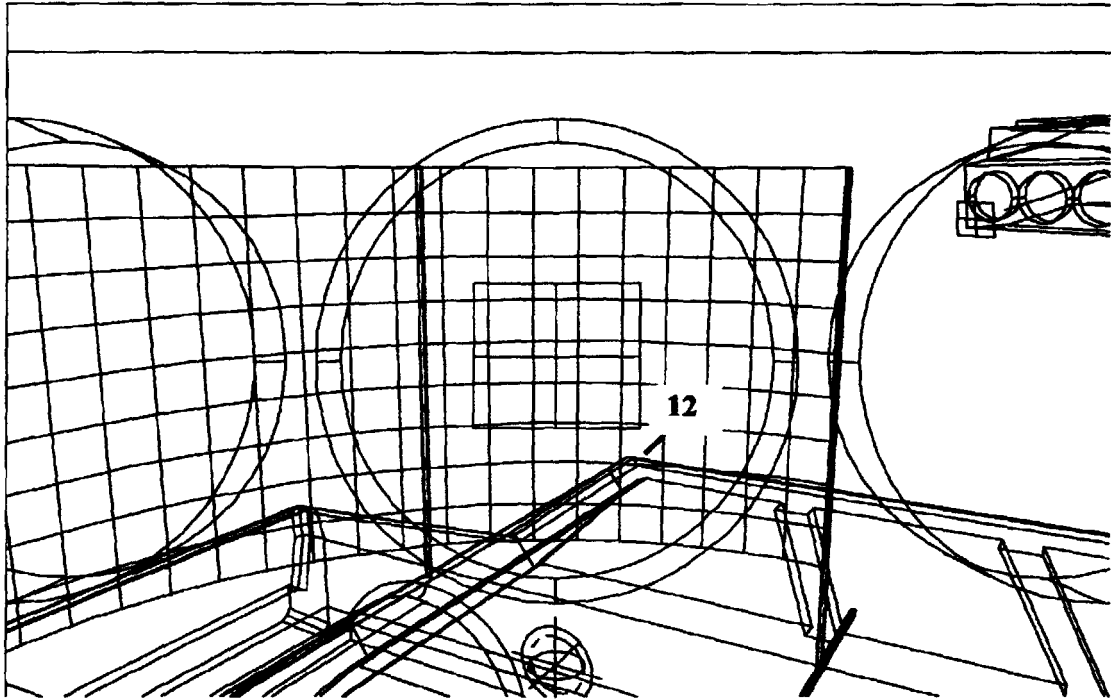
Figure 2: Field of view occlusion from vehicle cab.
