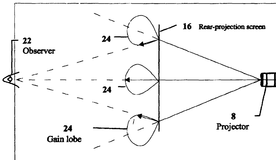
Figure 5: Rear-projection screen gain effect.
