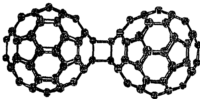
1, 2-( C_{60} ) 2 BY [2+2] CYCLIC ADDITION REACTION
