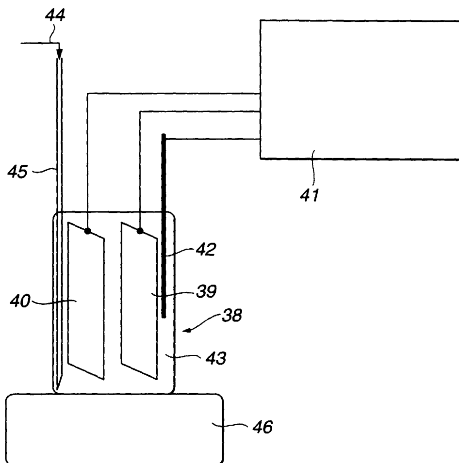
ELECTROLYTIC POLYMERIZATION APPARATUS
