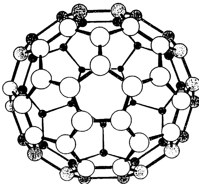
MOLECULAR STRUCTURE OF C 60
