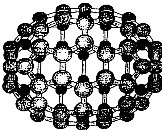
MOLECULAR STRUCTURE OF C 70
