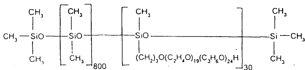
formula (X)
