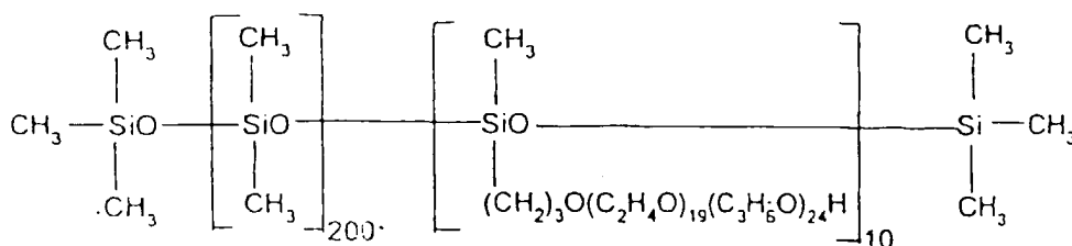
formula (V)
