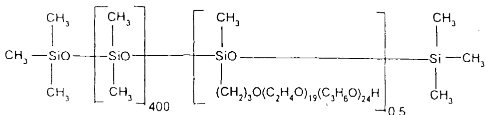
formula (VII)
