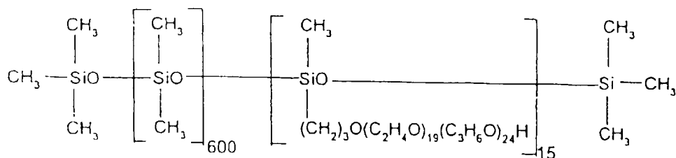
formula (IX)
