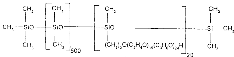
formula (VIII)
