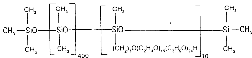
formula (IV)
