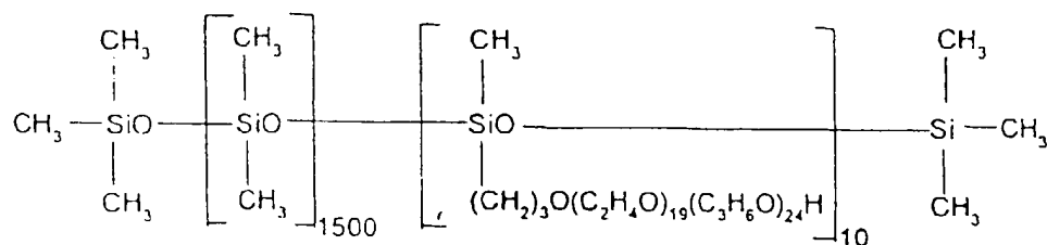
formula (VI)
