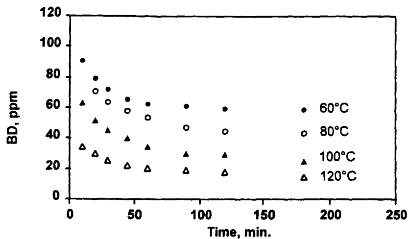
Figure 1. Effect of purging time and purging temperature on butadiene residue in CB: CB N550 purged at 60, 80, 100 and 120°C.
