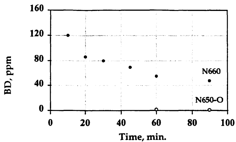
Figure 3. Oxidized CBs have low butadiene residue: CB N660 and oxidized CB N650-O.
