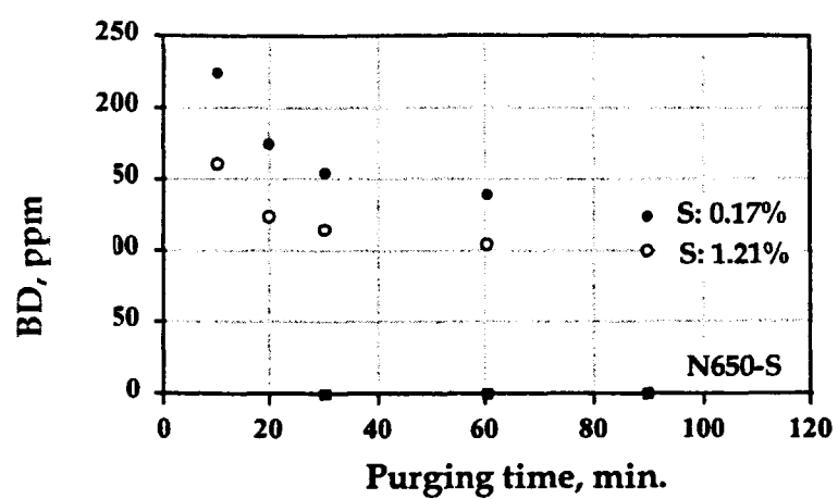
Figure 5. CB rich in sulfur as produced by CB manufacturer have high butadiene residue.
