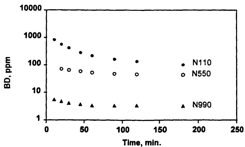
Figure 2. Desorption of butadiene from CB surface: N110, N550 and N990 purged at 80°C.
