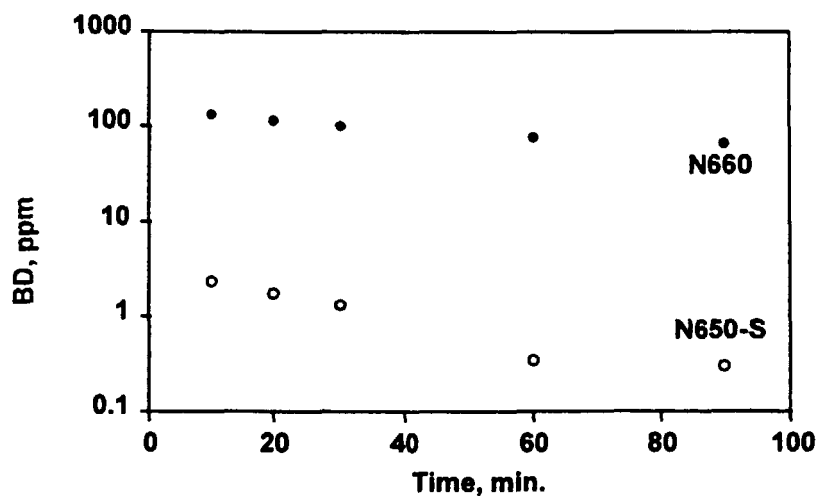
Figure 4. Butadiene adsorption decreases upon sulfur modification: N650-S: sulfur modified CB.
