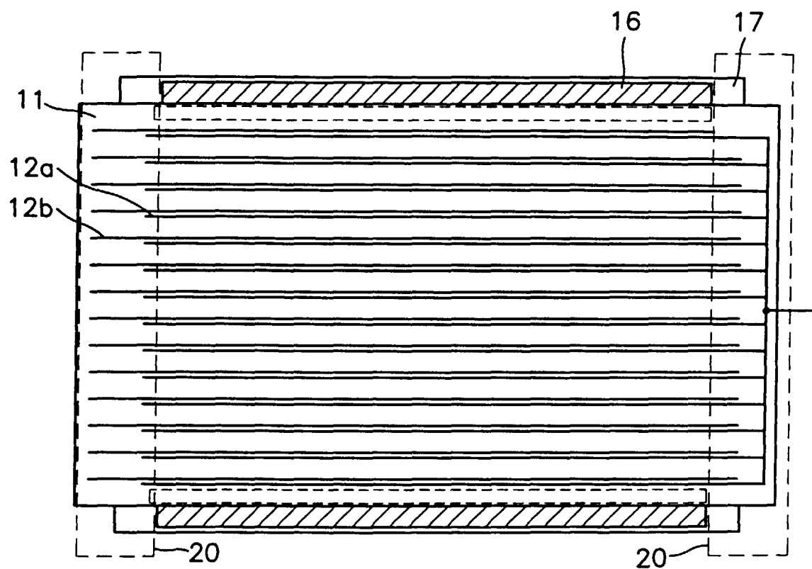
FIG. 6 (PRIOR ART)
