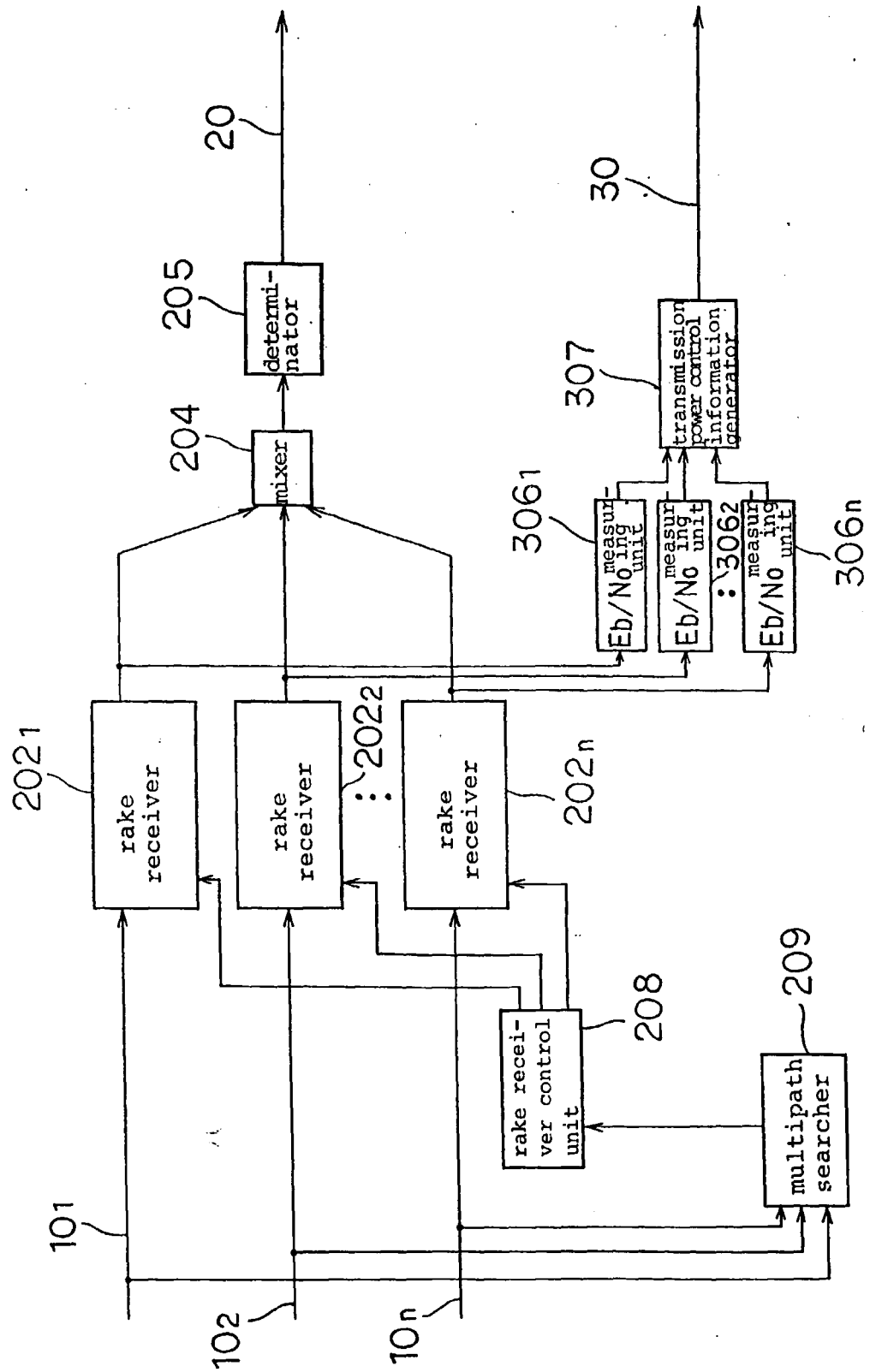
Fig. 2 PRIOR ART
