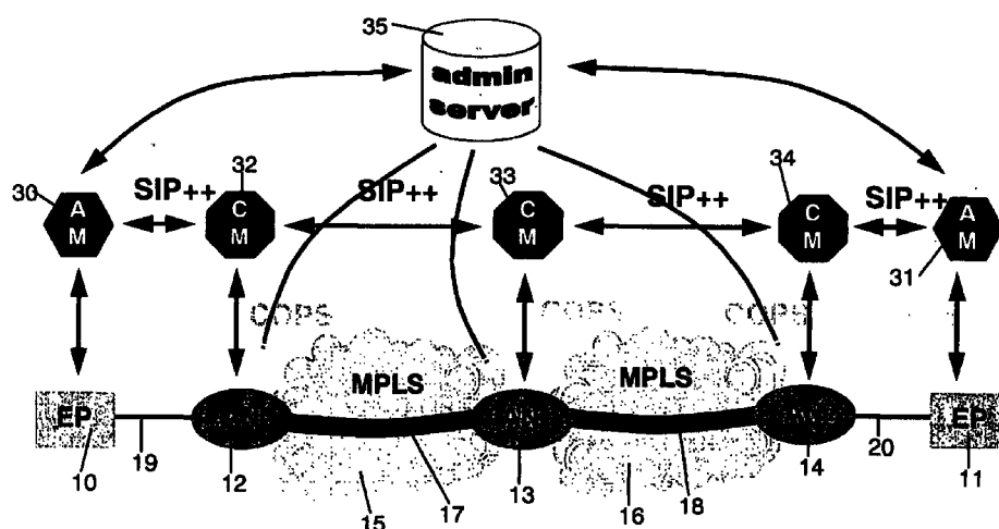
Figure 1 Configuration of network
