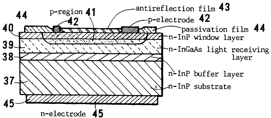
Fig. 7 PRIOR ART
