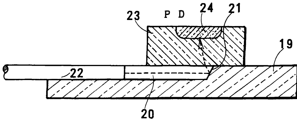
Fig. 4 PRIOR ART
