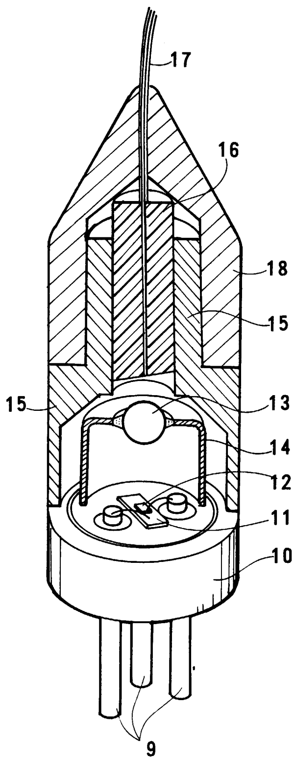
Fig. 3 PRIOR ART
