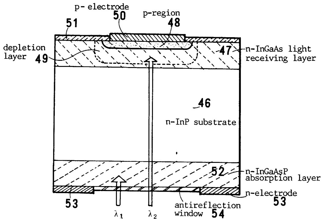
Fig. 9 PRIOR ART
