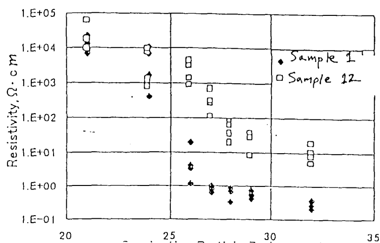
Electrically Conductive Particles (Vol%) Fig. 9
