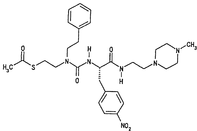
16) (2S)-2-[3-[2-(Acetylthio)ethyl]-3-phenethylureido]-N-[2-(4-methylpiperazin-1-yl)ethyl]-3-(4-nitrophenyl)propionamide
