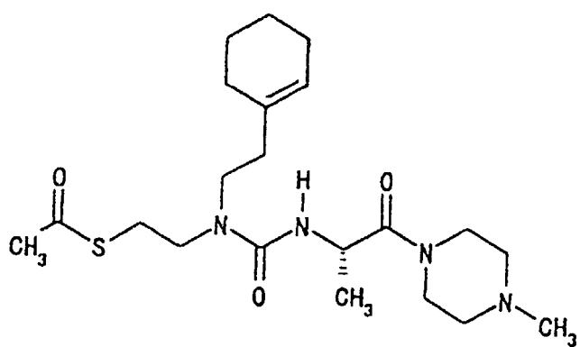
40 19) 1-[(2S)-2-[3-[2-(Acetylthio)ethyl]-3-[2-(cyclohexen-1-yl)ethyl]ureido]propionyl]-4-methylpiperazine
