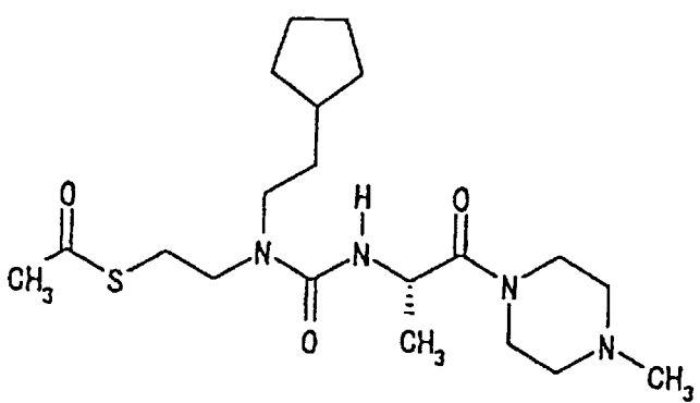
20 18) 1-[(2S)-2-[3-[2-(Acetylthio)ethyl]-3-(2-cyclopentylethyl)ureido]propionyl]-4-methylpiperazine
