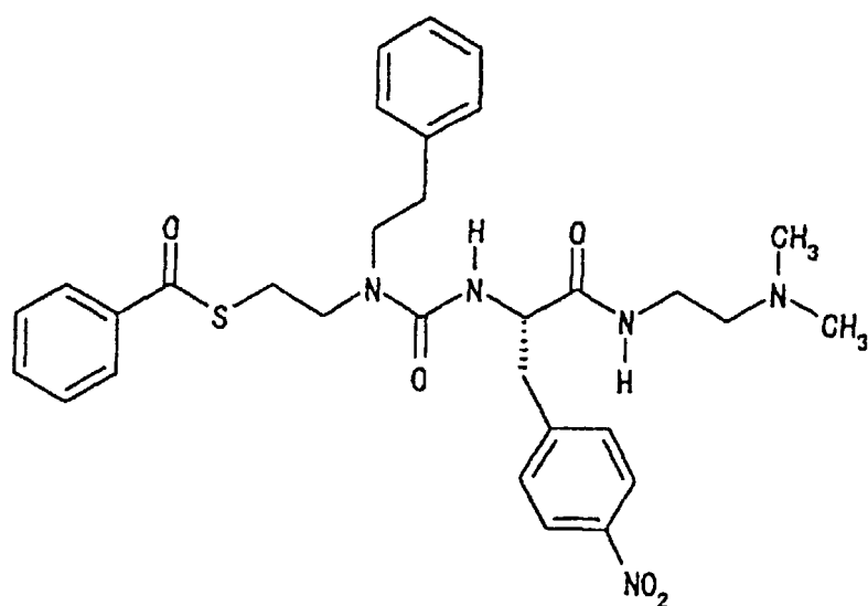
4) (2S)-2-[3-[2-(Benzoylthio)ethyl]-3-phenethylureido]-N-[2-(dimethylamino)ethyl]-3-(4-nitrophenyl)propionamide
