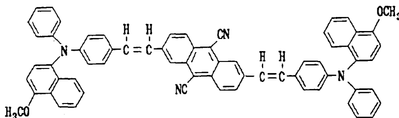
Structural Formula (7) - 2:
