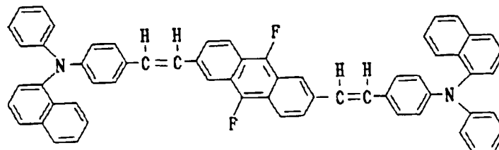
Structural Formula (7)-4:
