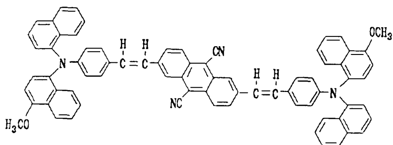
Structural Formula (7)-7:
