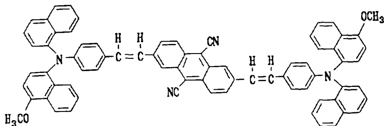
Structural Formula (7) - 7:
