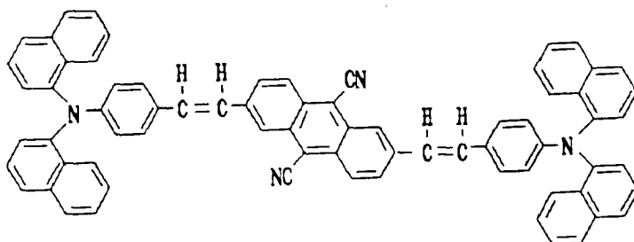
Structural Formula (7)-6:
