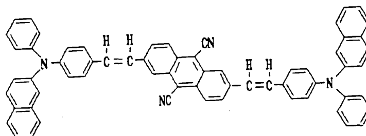
Structural Formula (7)-3:
