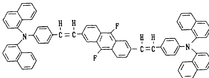
Structural Formula (7) - 8:
