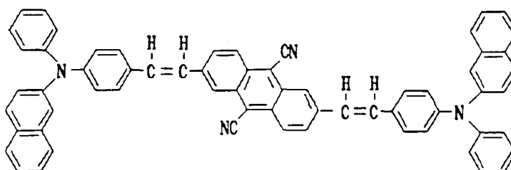
Structural Formula (7)-3:
