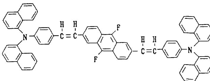
Structural Formula (7) - 8:
