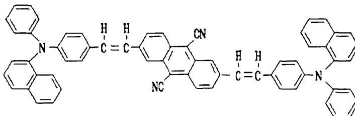
Structural Formula (7) - 1:
