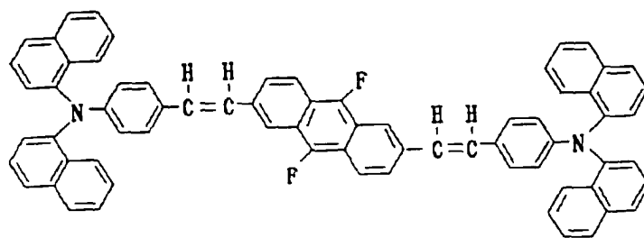
Structural Formula (7)-8:
