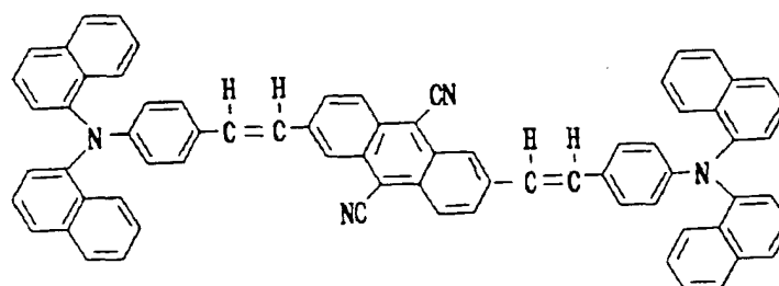
Structural Formula (7)-6:
