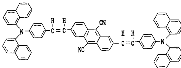
Structural Formula (7) - 6:
