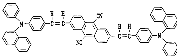
Structural Formula (7)-1:
