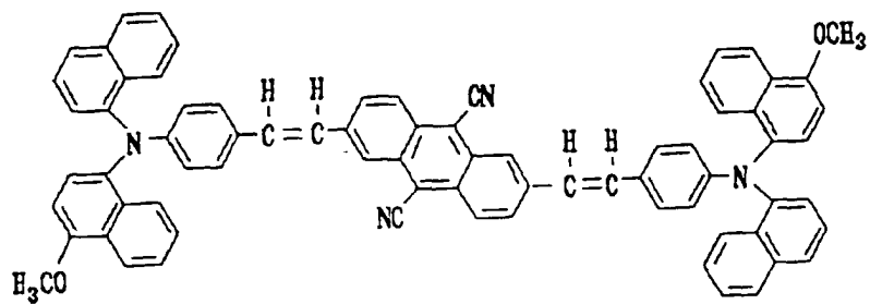
Structural Formula (7)-7:
