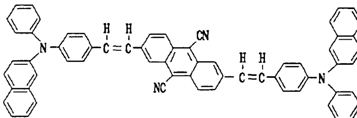
Structural Formula (7) - 3:
