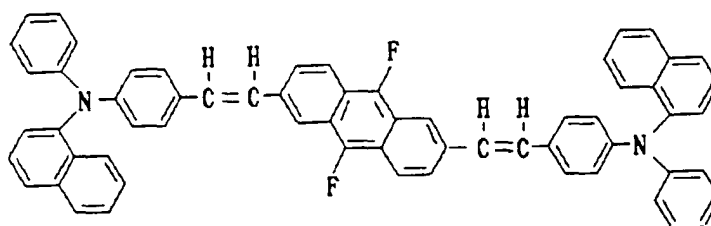
Structural Formula (7)-4:
