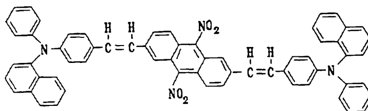
Structural Formula (7)-5:
