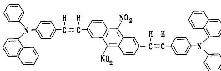
Structural Formula (7)-5:
