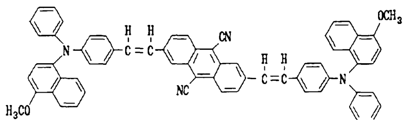
Structural Formula (7)-2:
