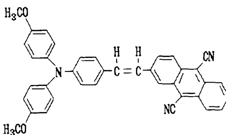
Structural Formula (20) - 5:
