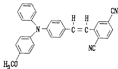
Structural Formula (20)-16:
