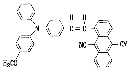
Structural Formula (20)-10:
