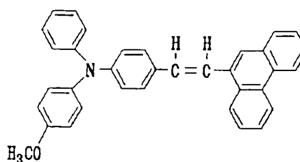
Structural Formula (20)-15:
