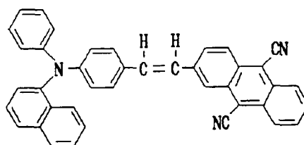
Structural Formula (20)-2:
