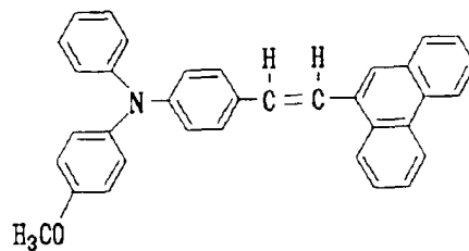
Structural Formula (20)-15:
