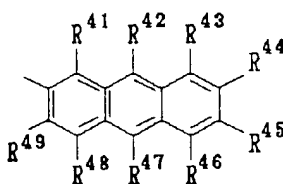
General Formula (8) :
