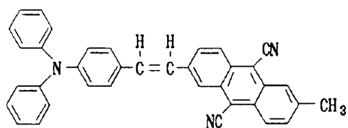
Structural Formula (20)-6:
