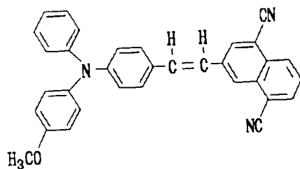
Structural Formula (20)-8:
