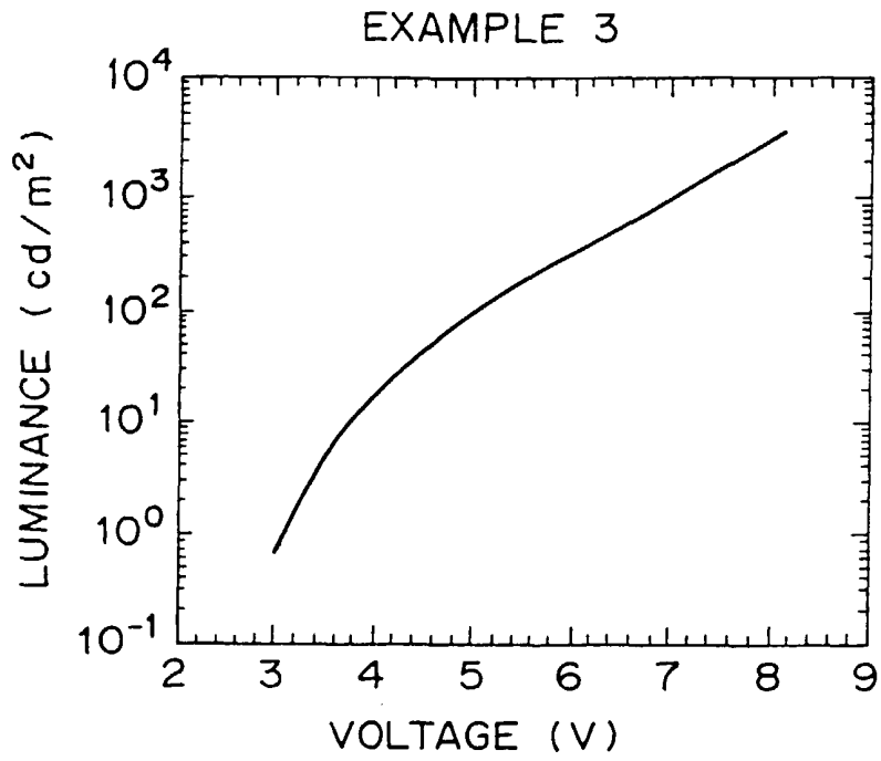
VOLTAGE - LUMINANCE CHARACTERISTIC
