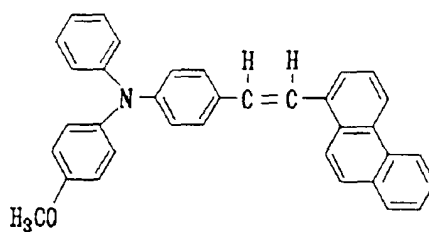
Structural Formula (20)-14:
