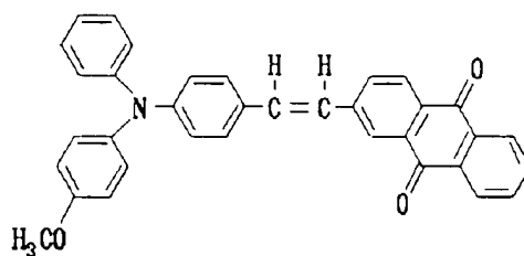
Structural Formula (20)-19:
