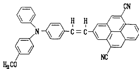
Structural Formula (20) -17:
