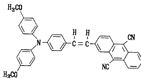
Structural Formula (20) -5:
