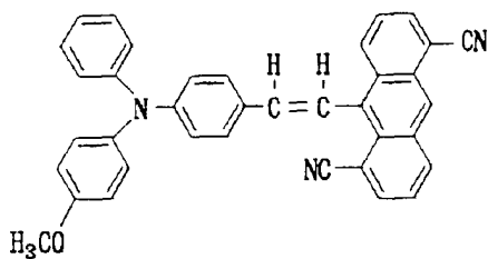
Structural Formula (20)-11:
