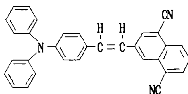
Structural Formula (20)-7:
