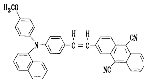
Structural Formula (20)-3:
