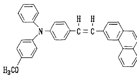
Structural Formula (20)-12:
