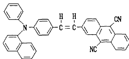
Structural Formula (20) - 2:
