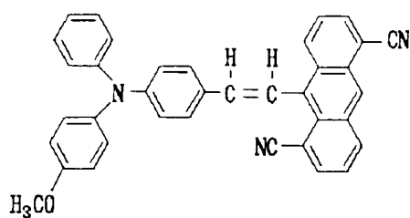
Structural Formula (20)-11:
