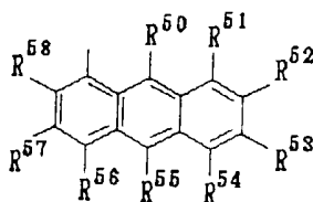
General Formula (9) :
