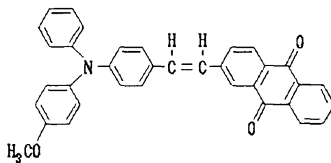
Structural Formula (20) -19:
