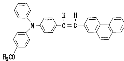
Structural Formula (20)-13:
