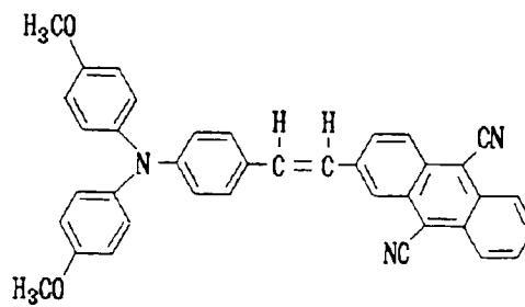
Structural Formula (20)-5:
