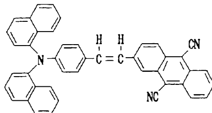
Structural Formula (20)-4:
