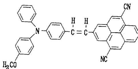
Structural Formula (20)-17:
