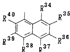
General Formula (7) :
