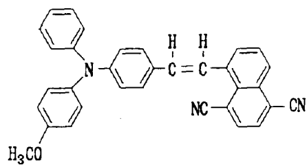
Structural Formula (20)-9:
