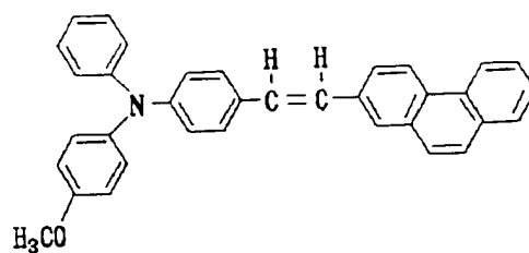
Structural Formula (20)-13:
