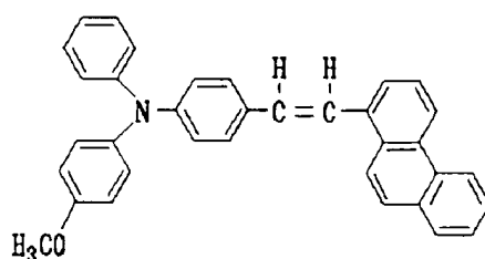
Structural Formula (20)-14:
