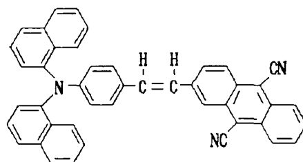
Structural Formula (20) -4:
