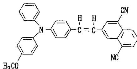
Structural Formula (20) - 8:
