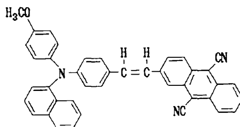
Structural Formula (20)-3:
