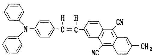
Structural Formula (20) - 6:
