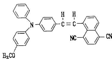
Structural Formula (20)-9:
