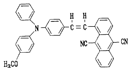
Structural Formula (20)-10:
