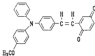
Structural Formula (20)-18:
