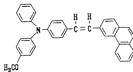
Structural Formula (20)-12:
