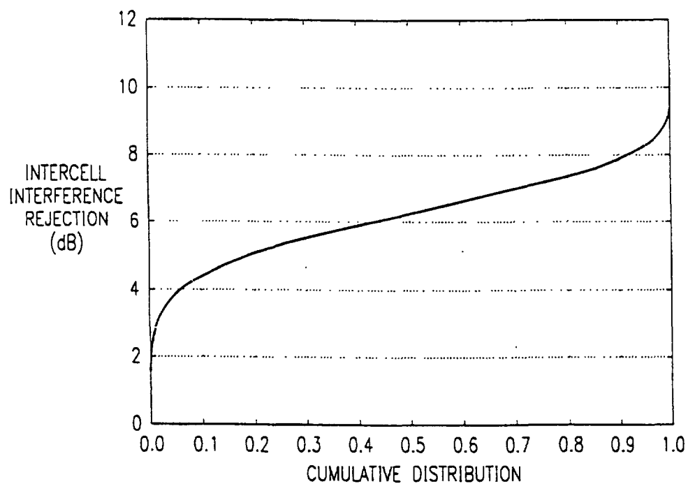
FIG. 6 (PRIOR ART)
