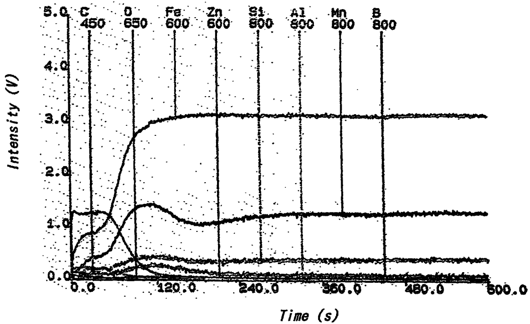
FIG. 8b Heat treatment (100%N 2 )
