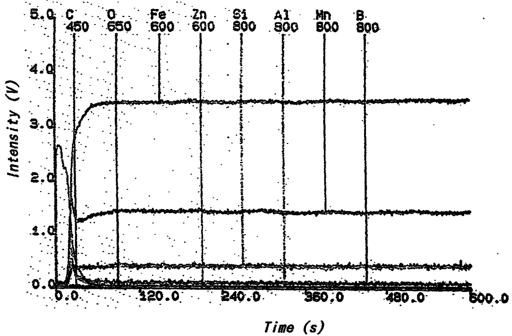
FIG. 7a No heat treatment
