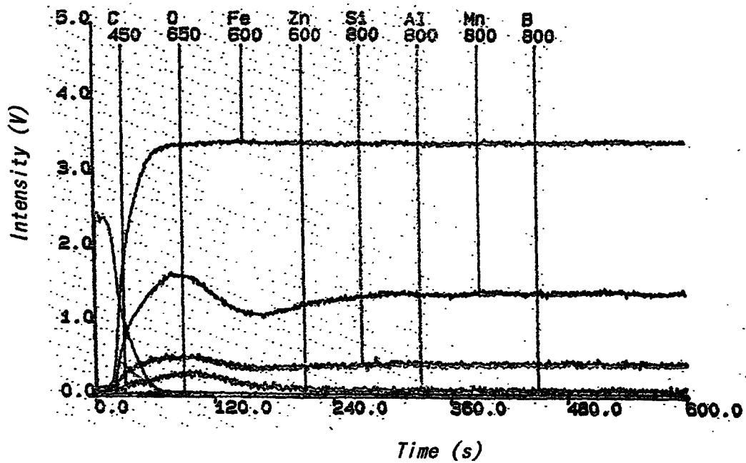
FIG. 7b Heat treatment (100%N 2 )
