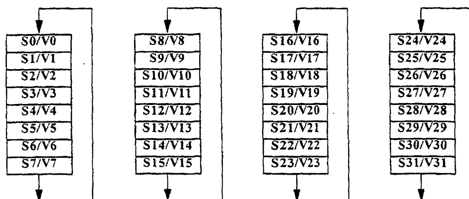
Illustration 2. Circulating Single Precision Registers
