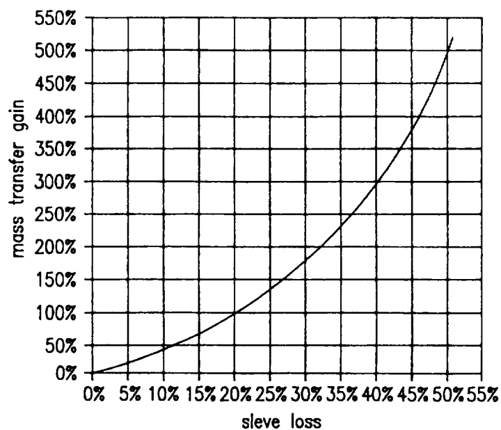
Mass transfer gain vs sieve loss for a composite adsorbent bead
