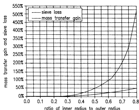
Mass transfer gain and sieve loss as function of inner to outer radius ratio for a composite adsorbent bead
