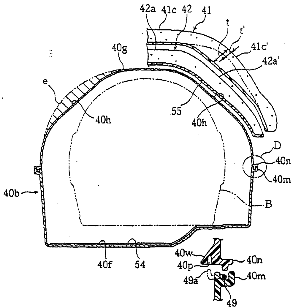
Enlarged and exploded view of D
