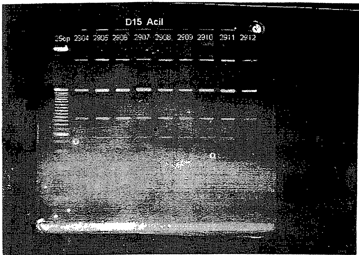
Figure 1 : Photographs of the electrophoresis gels obtained in the RFLP analysis of BASB027
