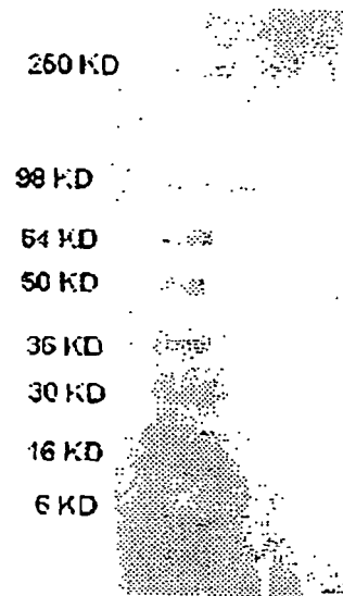
Figure 5: Western blot with tetra-His antibody of purified BASB027 protein.
