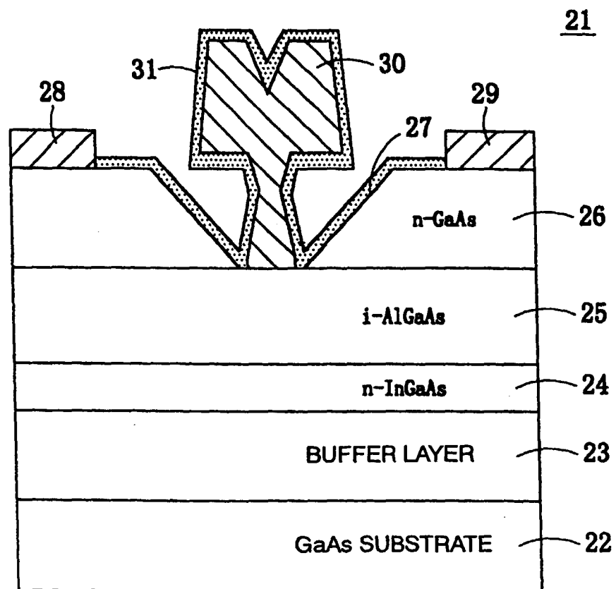
FIG. 2 PRIOR ART
